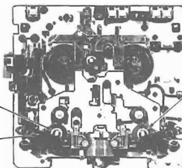
Pinch roller ass'y (F) [RXL0124]
