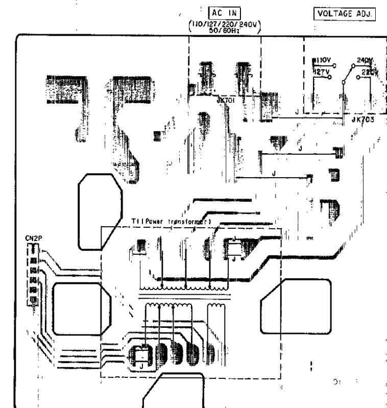
B POWER SUPPLY P.C.B. For (GC, PX) areas.
