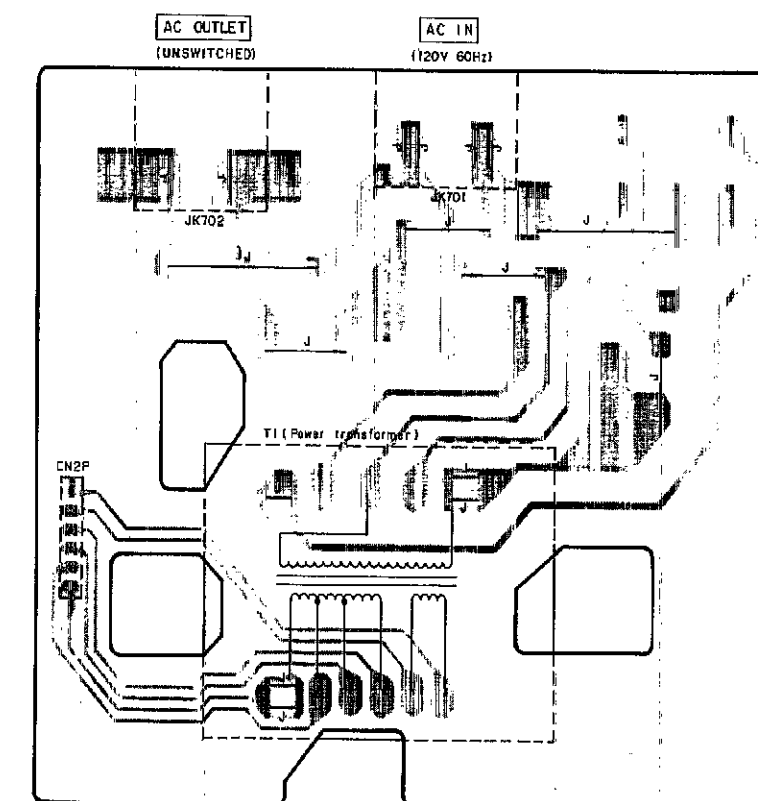
B POWER SUPPLY P.C.B. For (P, PC) areas.
