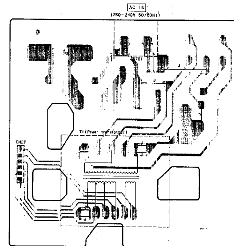
B POWER SUPPLY P.C.B. For (EB, EG, GN) areas.
