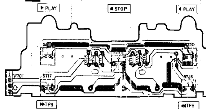
G OPERATION (DECK1) P.C.B.
