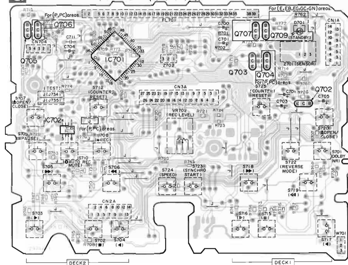
G OPERATION P.C.B. (REP1805A-S... (P,PC) REP1805D-S... (E,EB,EG,GC,GN))
