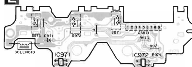
E MECHANISM P.C.B. (DECK1) (REP1655A)
