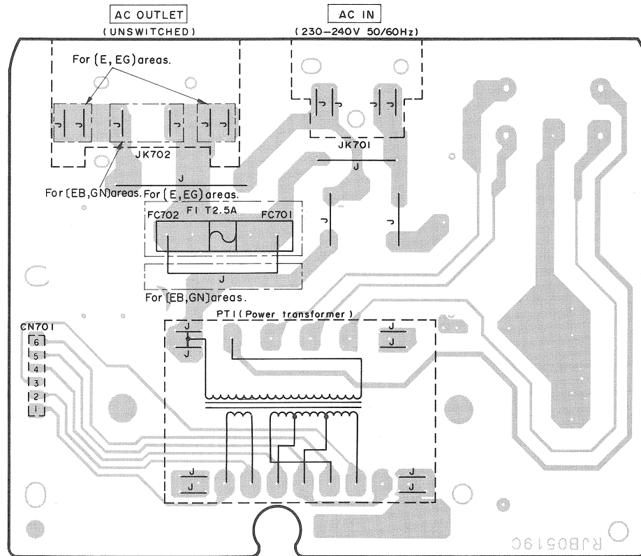
B POWER SUPPLY P.C.B. For [E, EB, EG, GN] areas.
