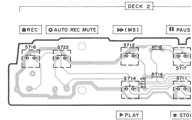
F OPERATION P.C.B.
