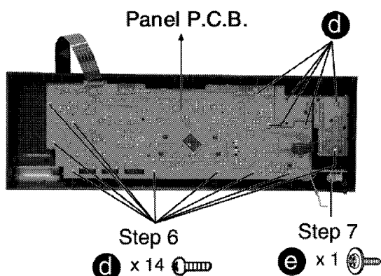
Step 6 & 7 Remove all the screws.
