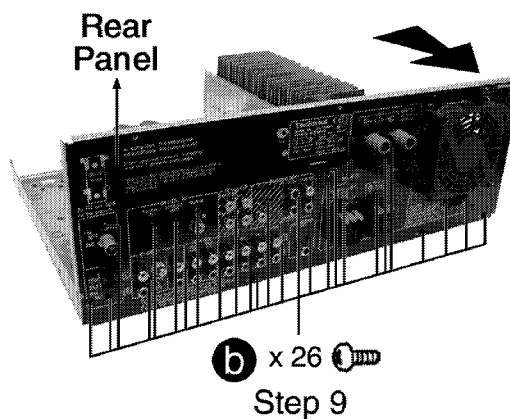
Step 9 Remove all the screws.
