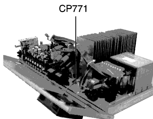
Step 10 Release the connector CP771.
