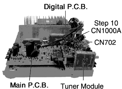
Step 11 Release the connectors CN702 and CN1000A. Pull up the Digital P.C.B. as shown.
