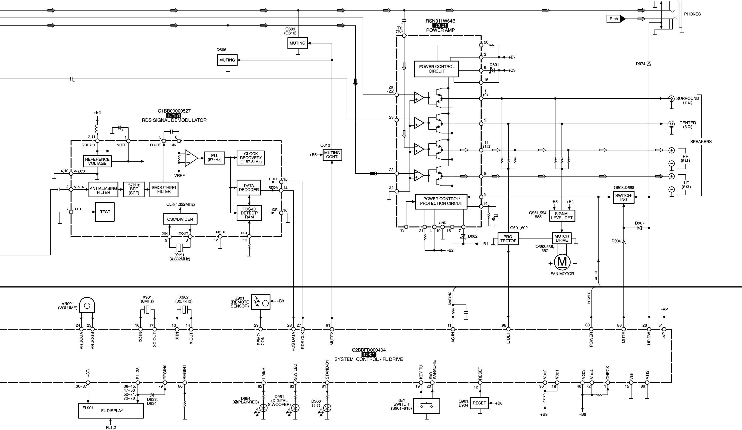
SA-EH790(E,EB,EG,EP) BLOCK DIAGRAM
