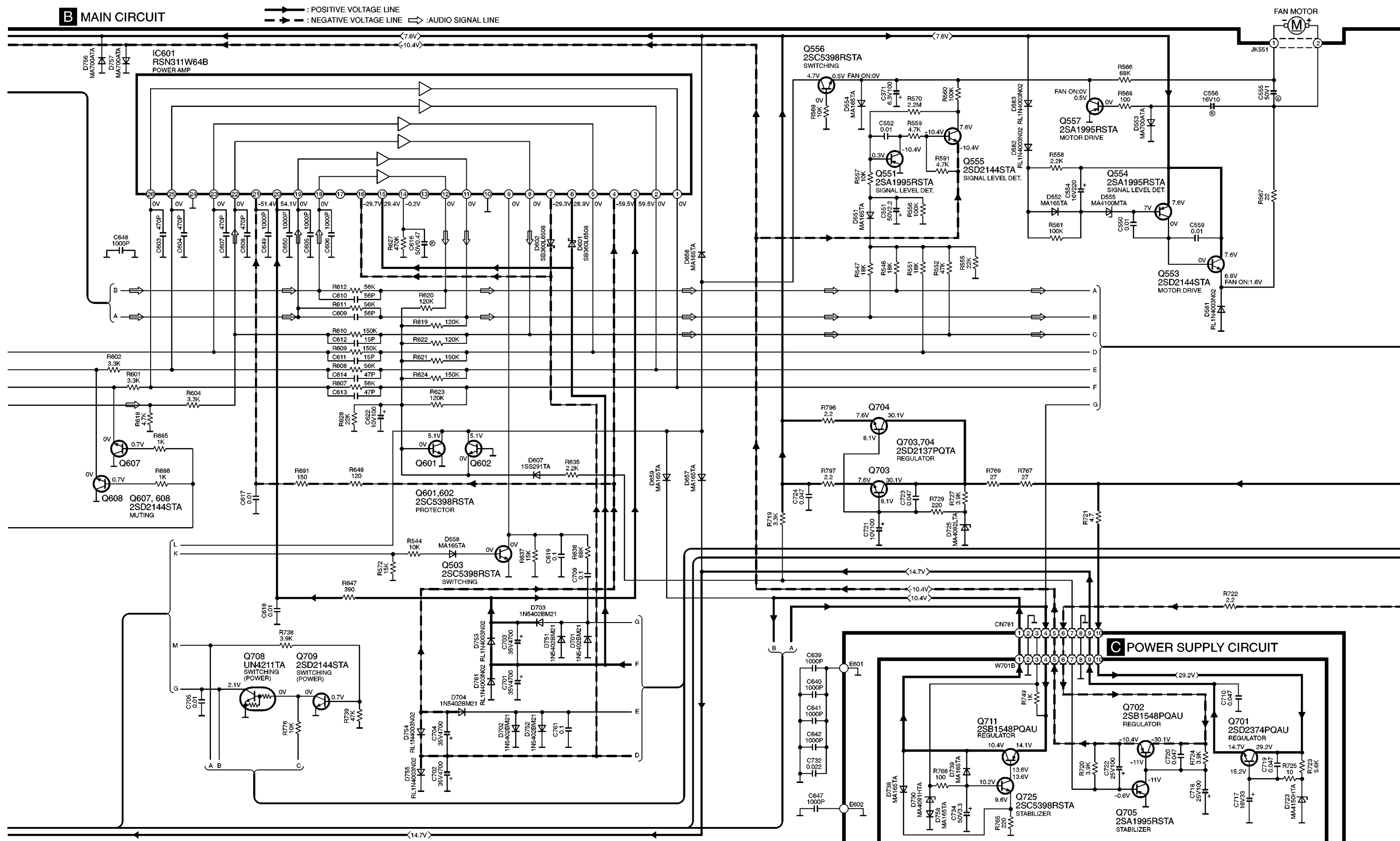
SA-EH790(E,EB,EG,EP) MAIN,POWER SUPPLY CIRCUIT DIAGRAM
