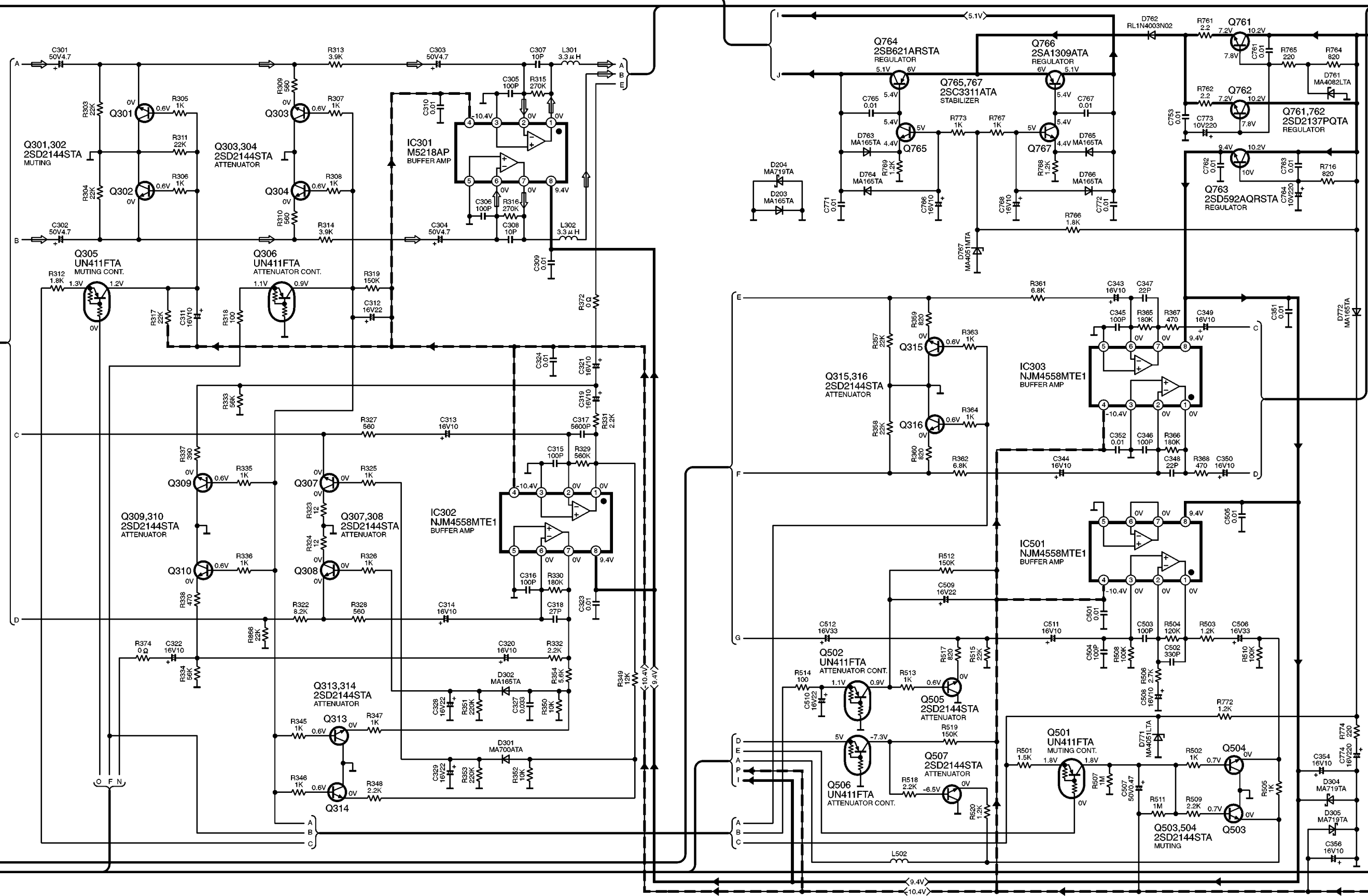
SH-DV280(EG) MAIN CIRCUIT DIAGRAM
