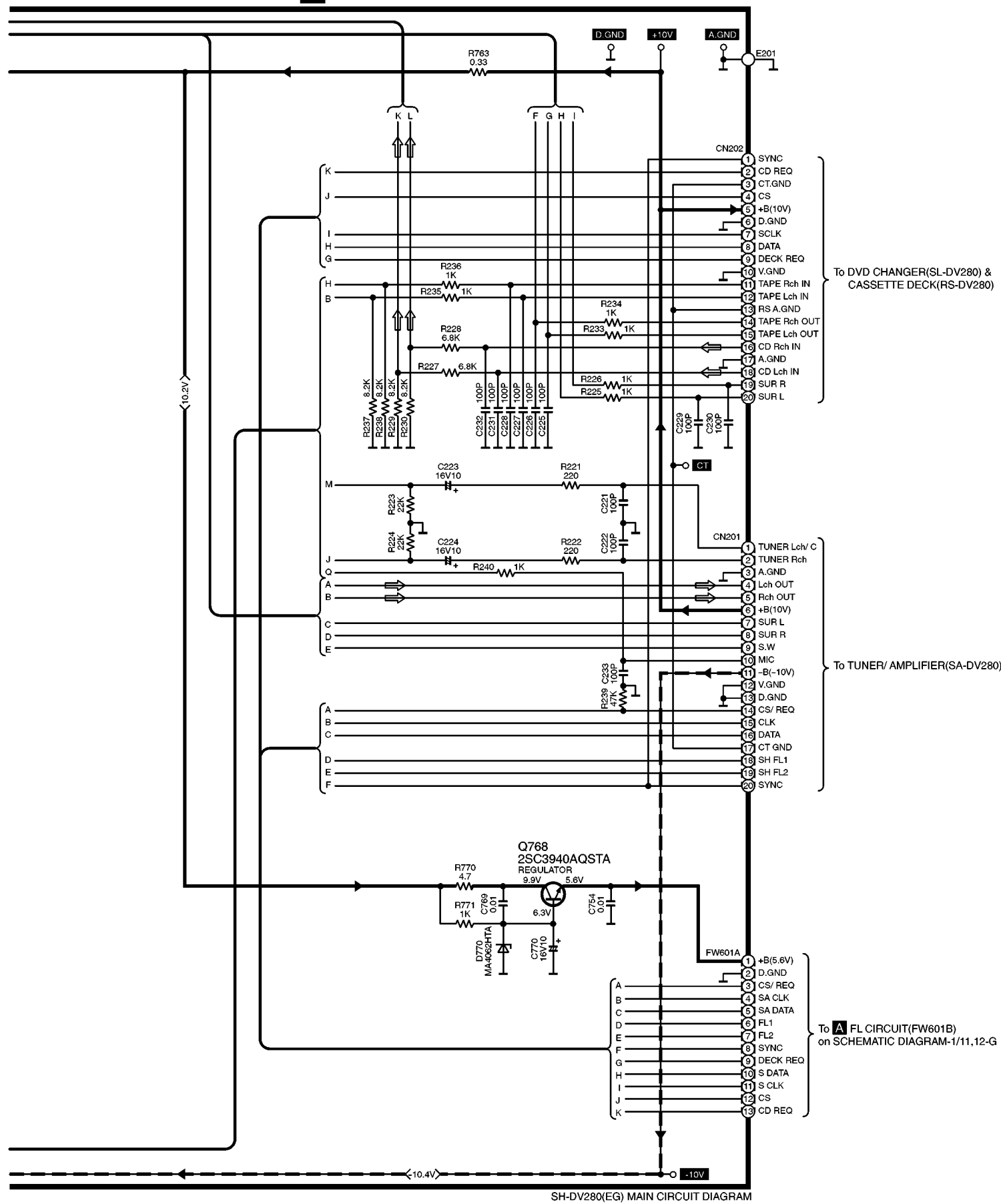
SH-DV280(EG) MAIN CIRCUIT DIAGRAM
