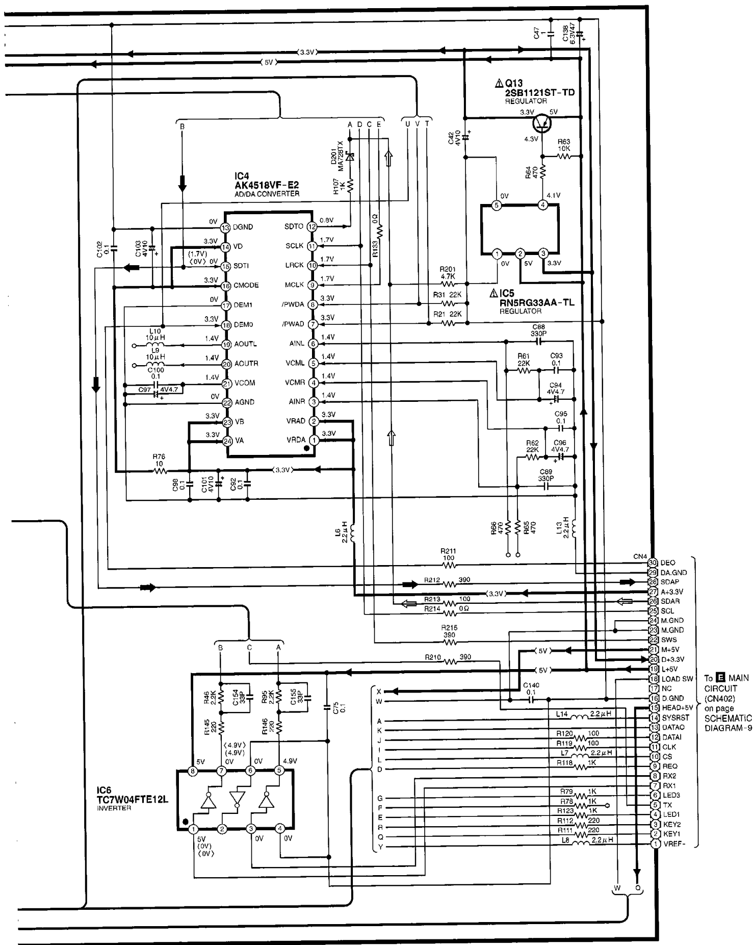
SCHEMATIC DIAGRAM-6
