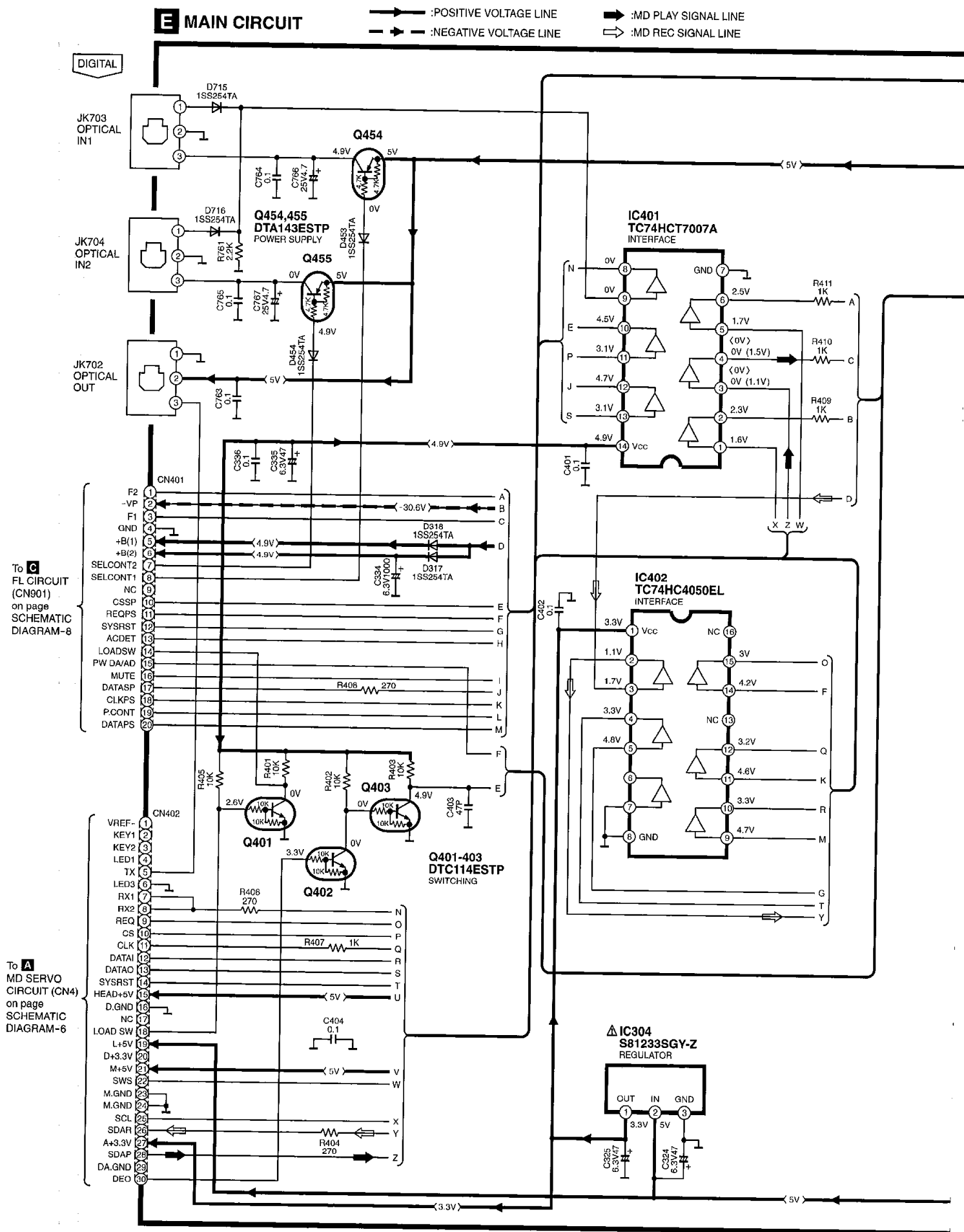
SCHEMATIC DIAGRAM-9
