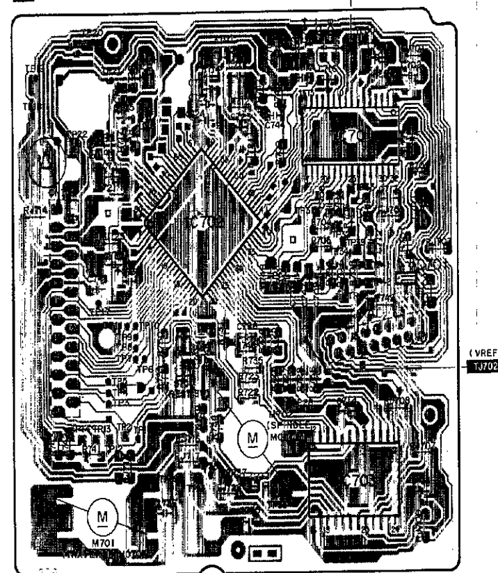
A SERVOP.C.B. (REP1650A-N)
