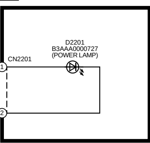
L LED CIRCUIT
