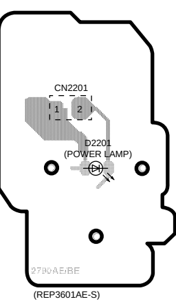
L LED P.C.B.
