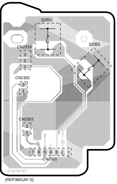
K LOADING MOTOR P.C.B.
