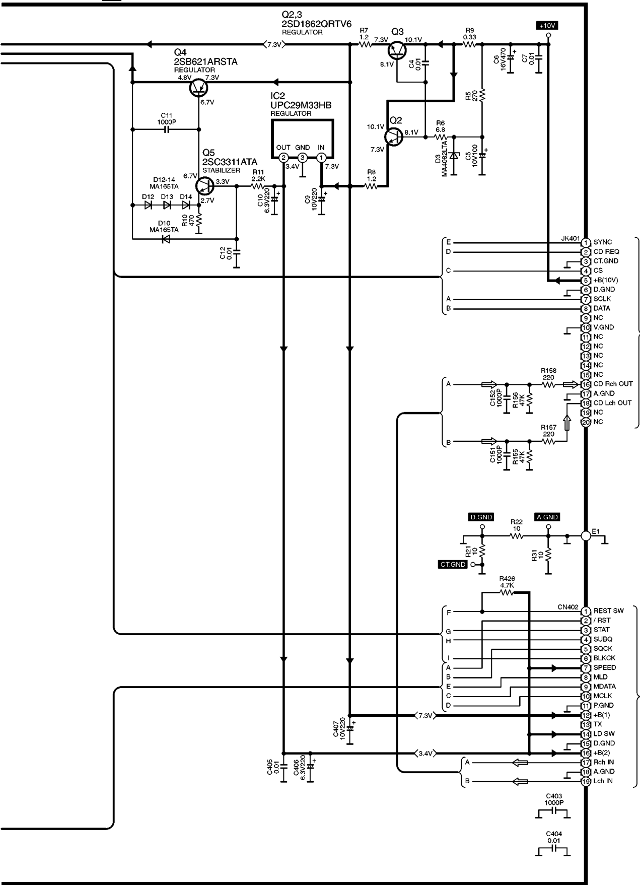
SL-EH590(EG) MAIN CIRCUIT DIAGRAM
