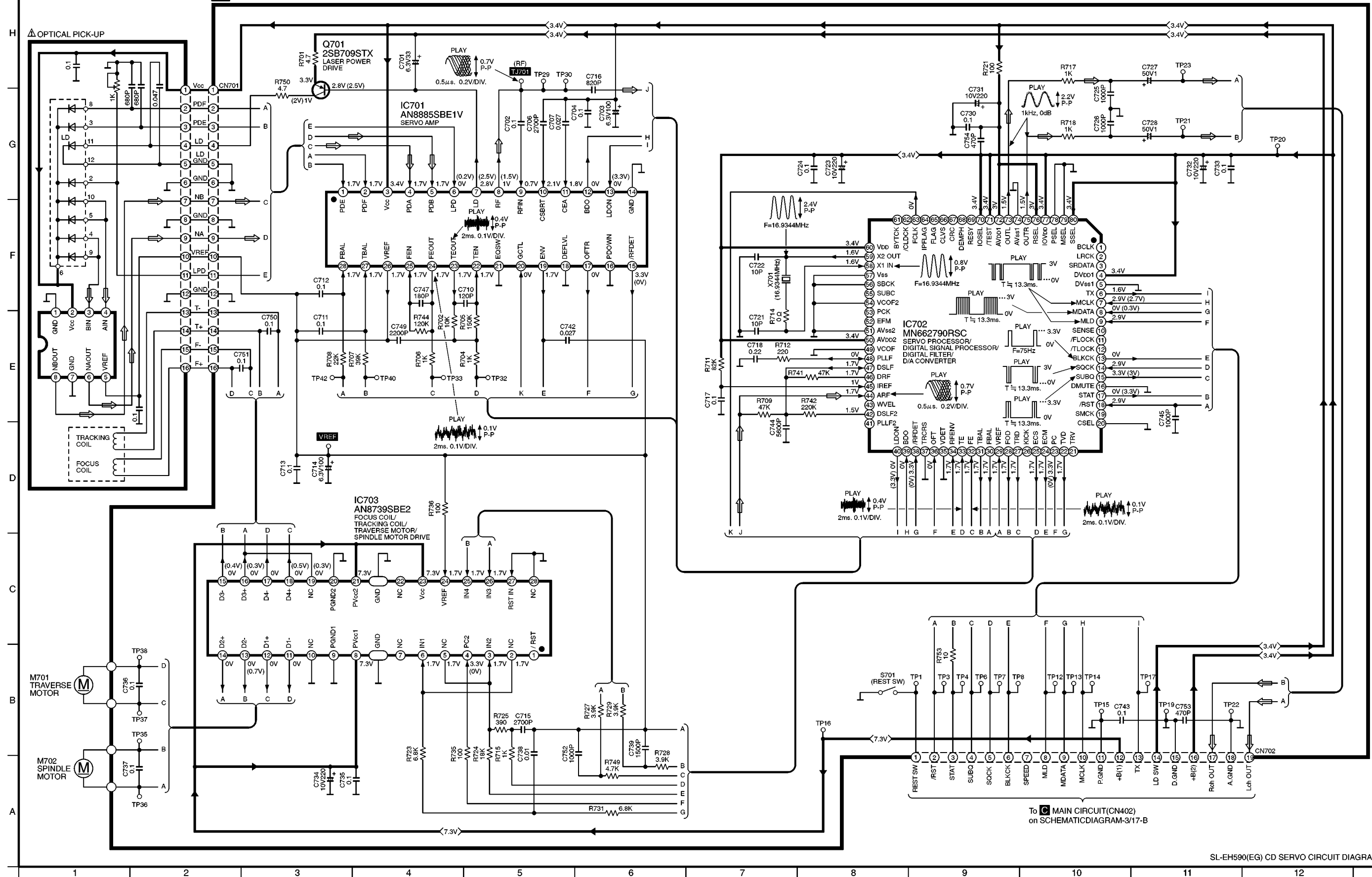
SCHEMATIC DIAGRAM-1
