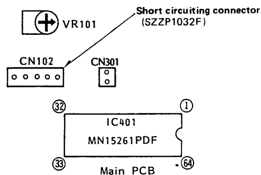
Main PCB
