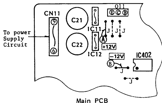
Main PCB
