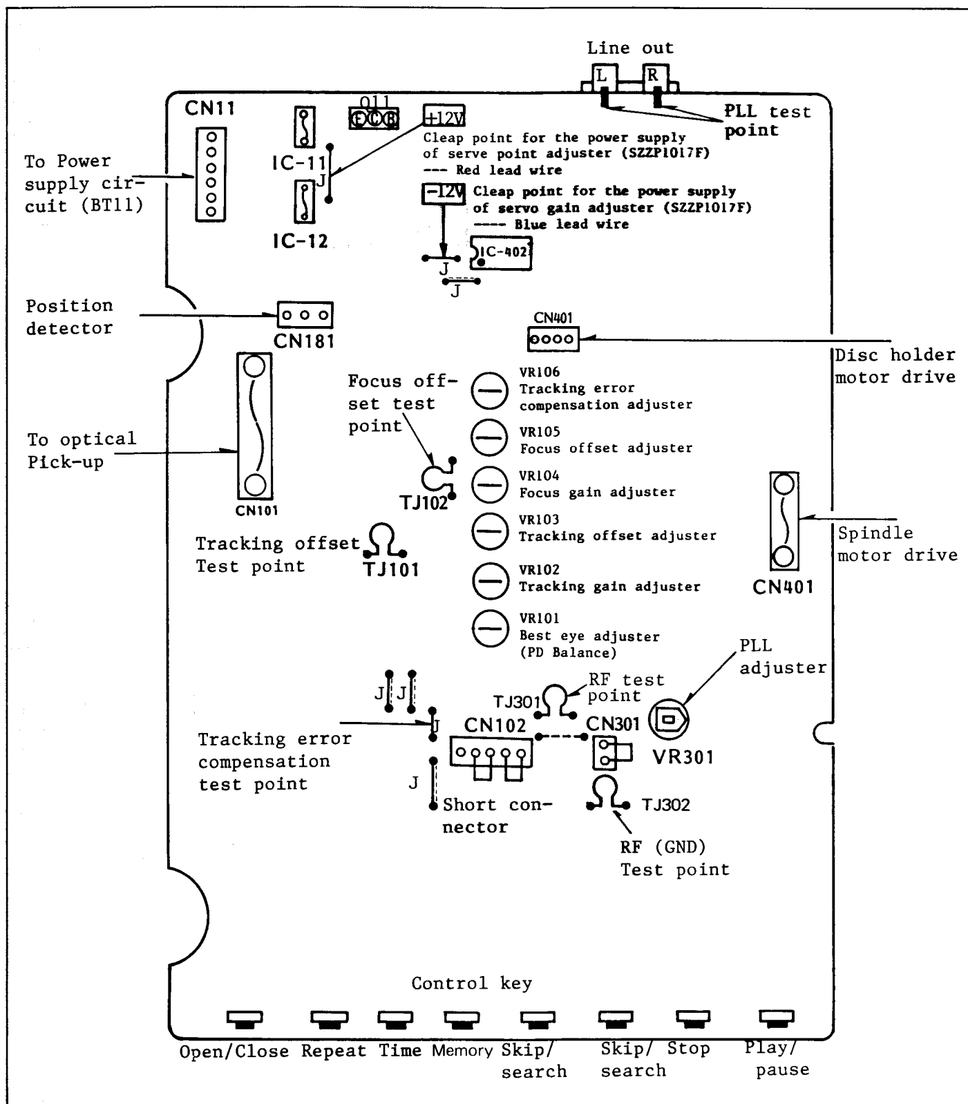
Main circuit
