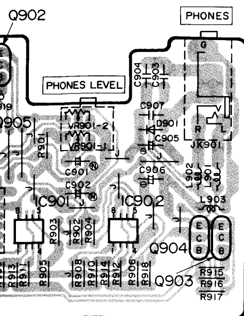
HEADPHONES P.C.B.
