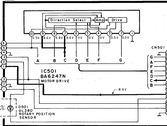
E OPERATION CIRCUIT (P.C. Board: on pages 41, 42)
