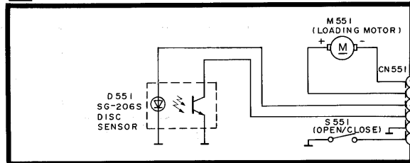
G SENSOR CIRCUIT (P.C. Board: on page 43)
