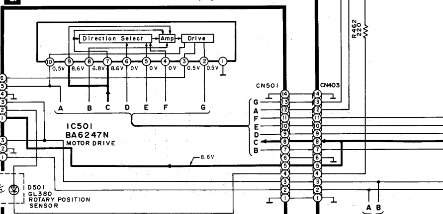
E OPERATION CIRCUIT ( P.C.Board : on pages 43,44 )
