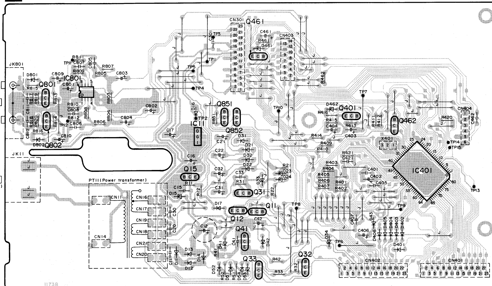
H MAIN P.C.B.(REP2073A-M)
