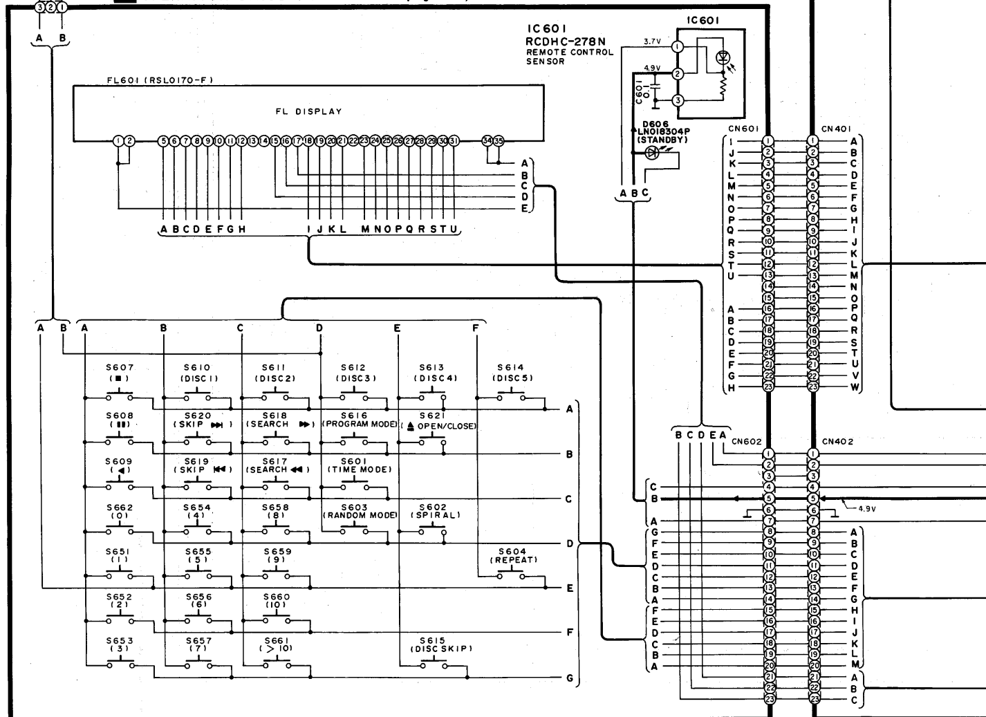
E OPERATION CIRCUIT ( P.C.Board : on pages 43,44 )
