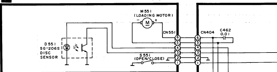
G SENSOR CIRCUIT (P.C.Board: on page 44)
