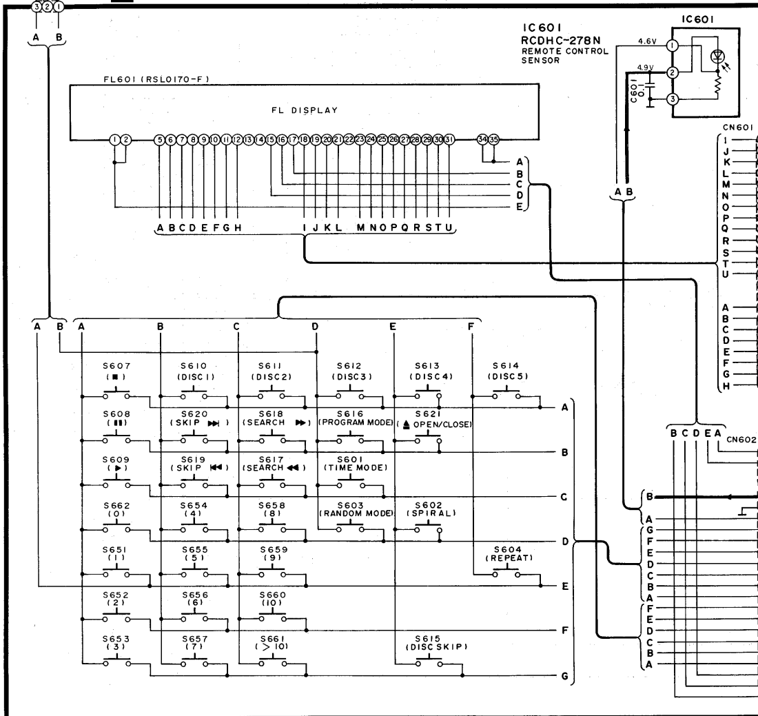
E OPERATION CIRCUIT (P.C. Board: on pages 41, 42)
