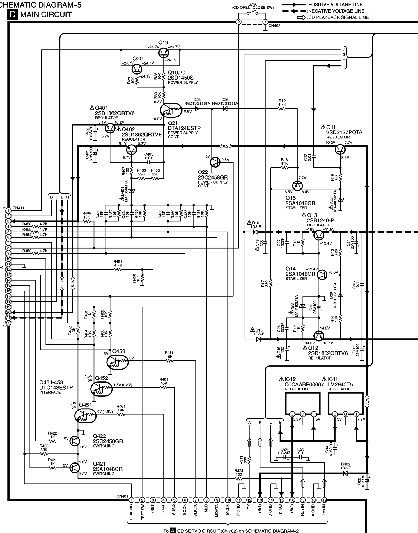
SCHEMATIC DIAGRAM-5
