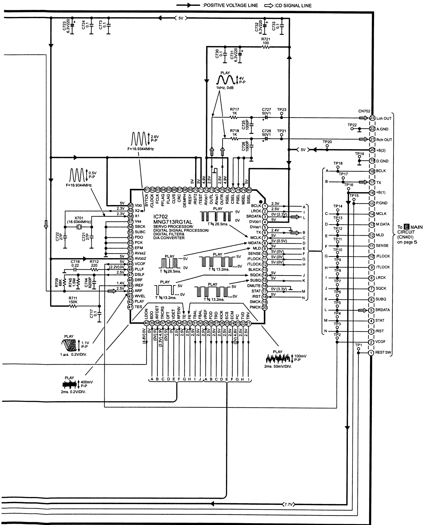
SCHEMATIC DIAGRAM-2
