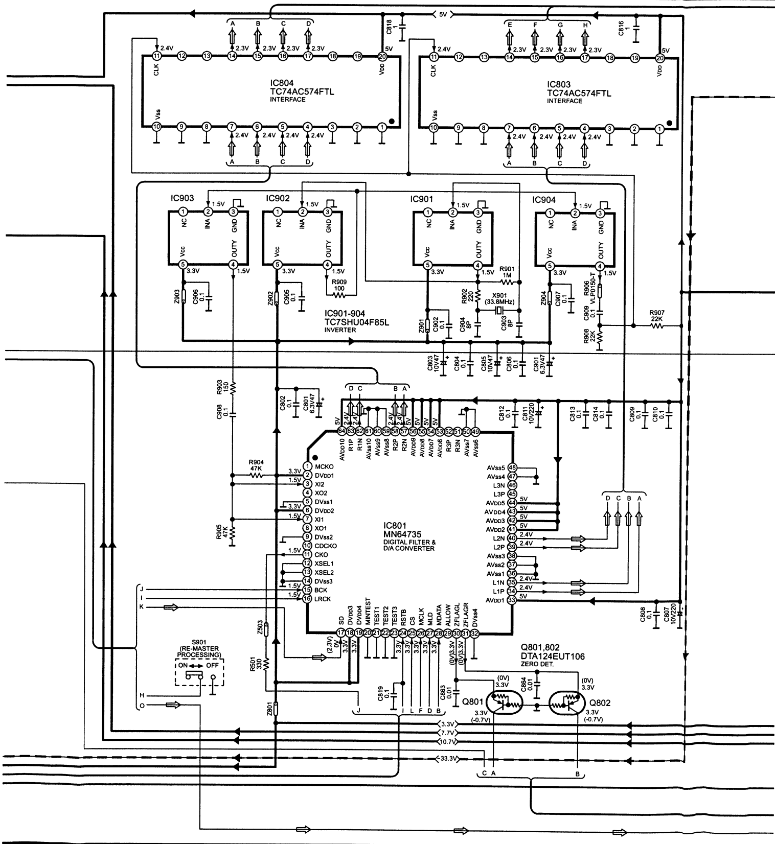
SCHEMATIC DIAGRAM-6
