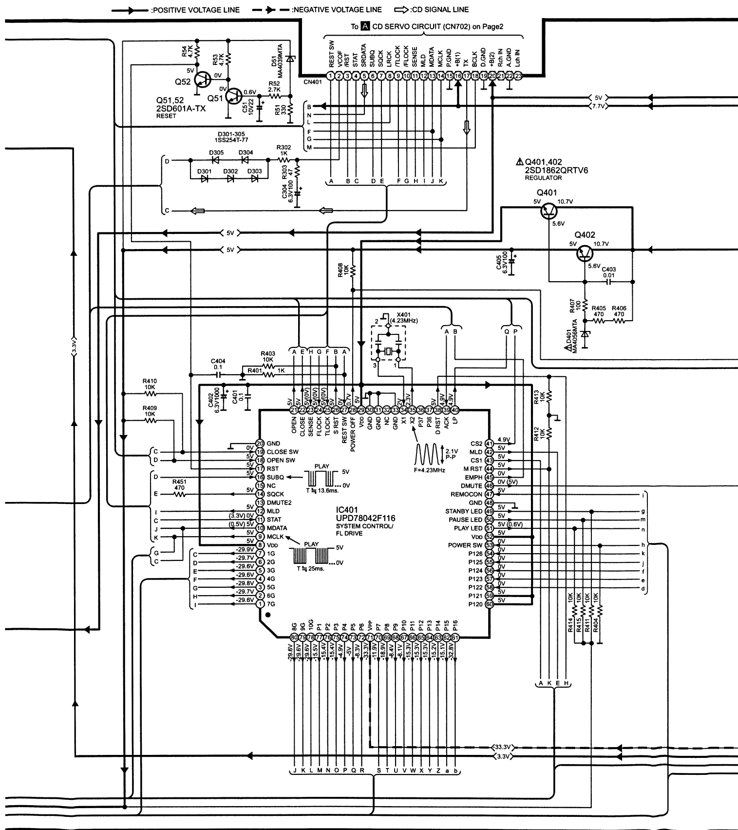
SCHEMATIC DIAGRAM-5
