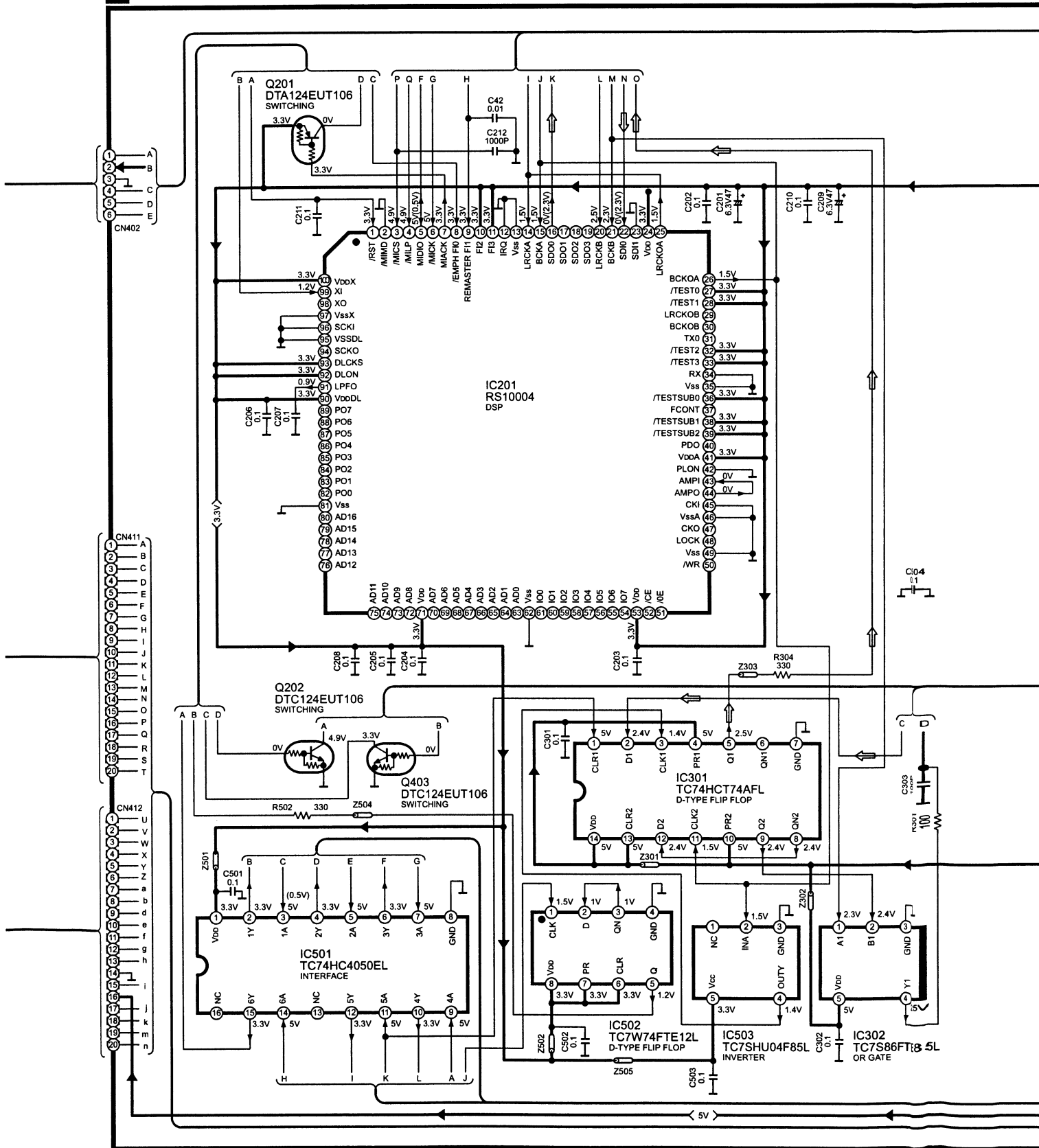
SCHEMATIC DIAGRAM-4
