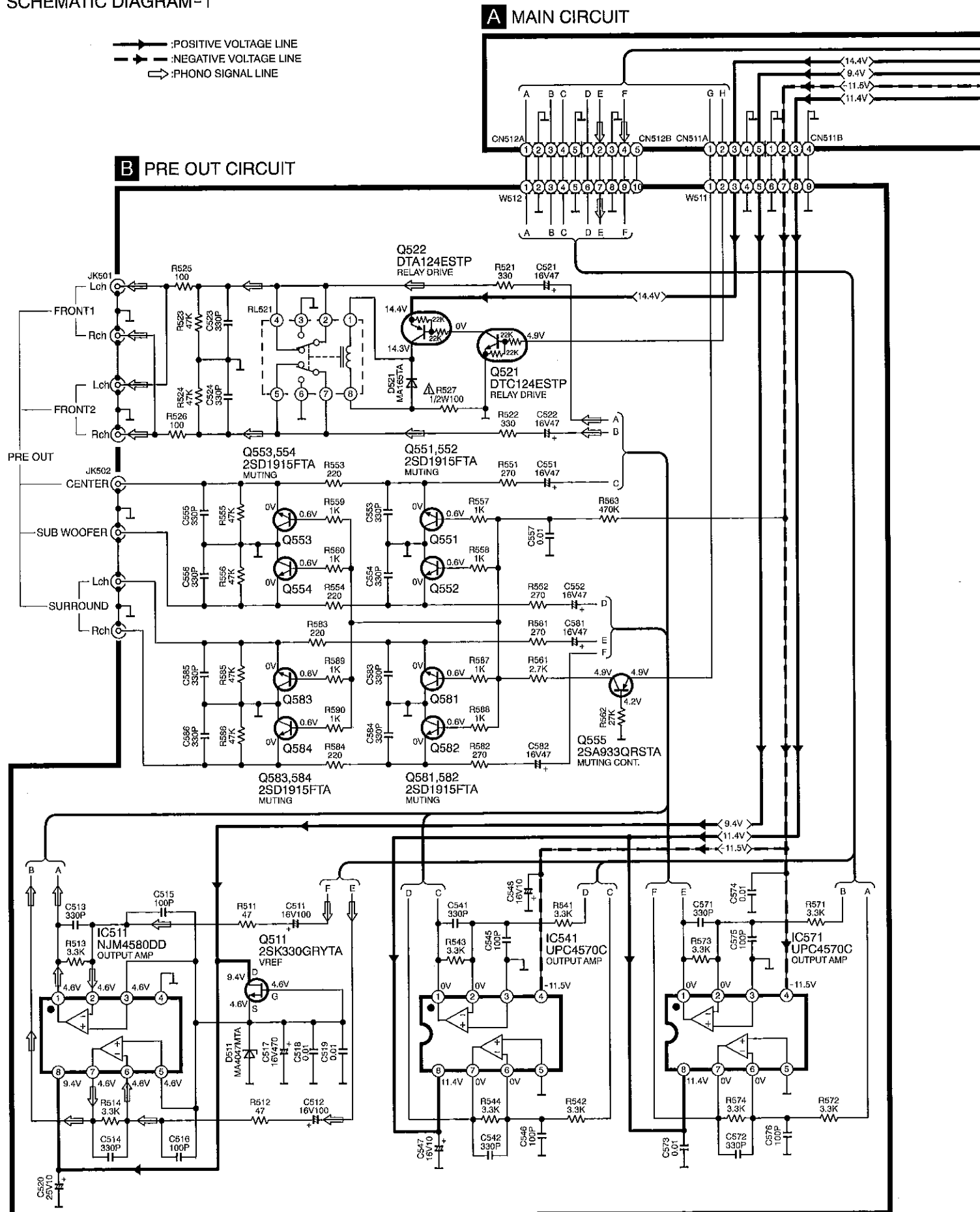
SCHEMATIC DIAGRAM-1
