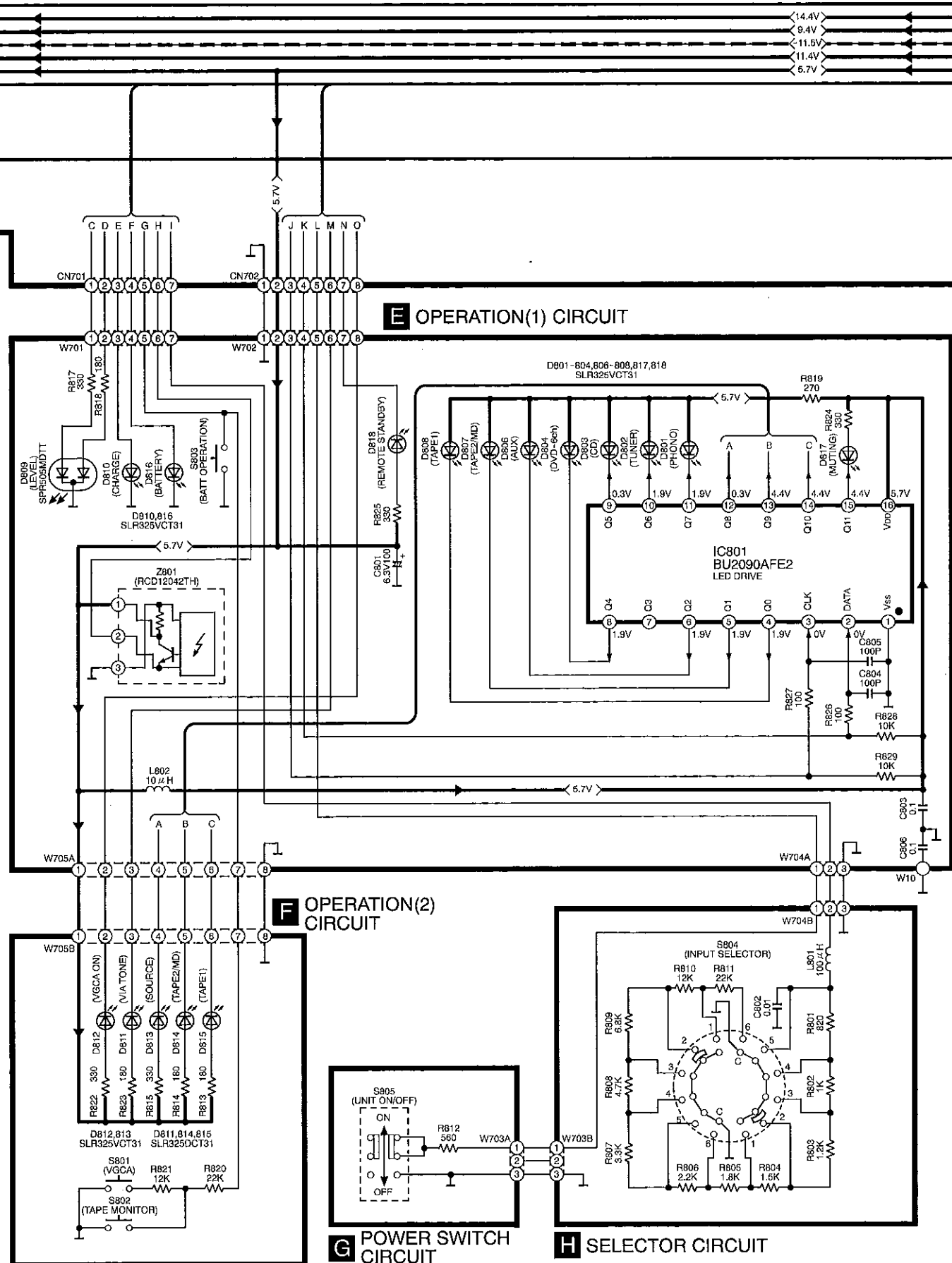
SCHEMATIC DIAGRAM-5
