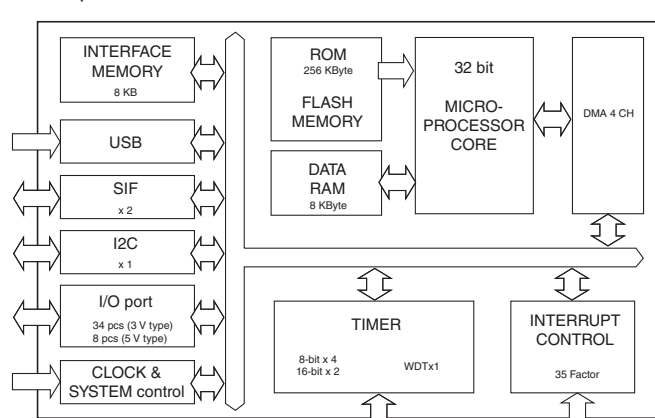
IC604: MN103FBSKYAA Microprocessor
