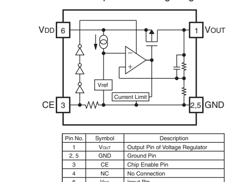
IC608: R1172S331B-E2-F CMOS-based positive-voltage regulator IC
