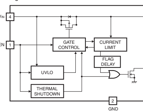
IC606: R5523N001A-TR-F High side switch IC
