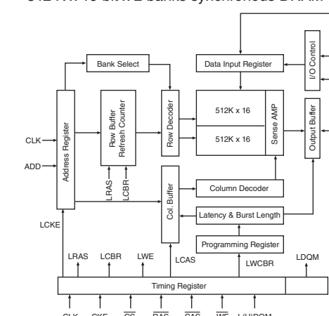
IC605: M12L16161A-TTG 512 K x 16-bit x 2 banks synchronous DRAM
