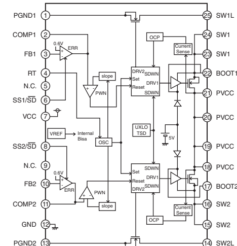
IC607: BD9302FP-E2 2.5 MHz 2 A power switch 2 ch step-down switching regulator
