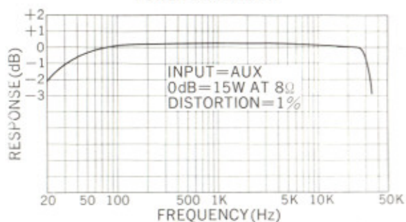
POWER BANDWIDTH
