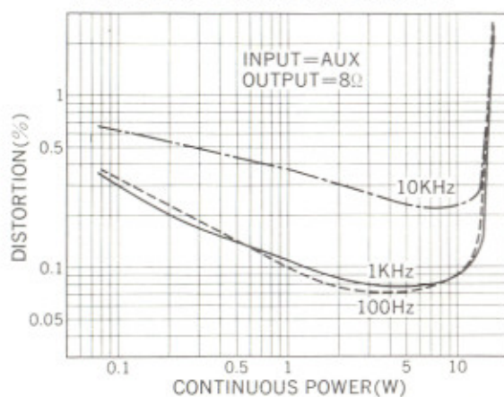
POWER OUTPUT HARMONIC DISTORTION
