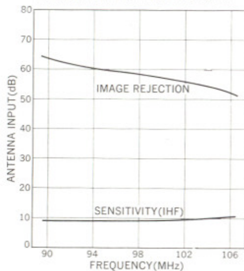
FM SENSITIVITY & IMAGE REJECTION
