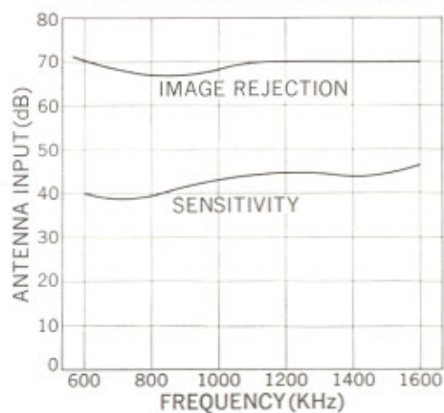
AM SENSITIVITY & IMAGE REJECTION
