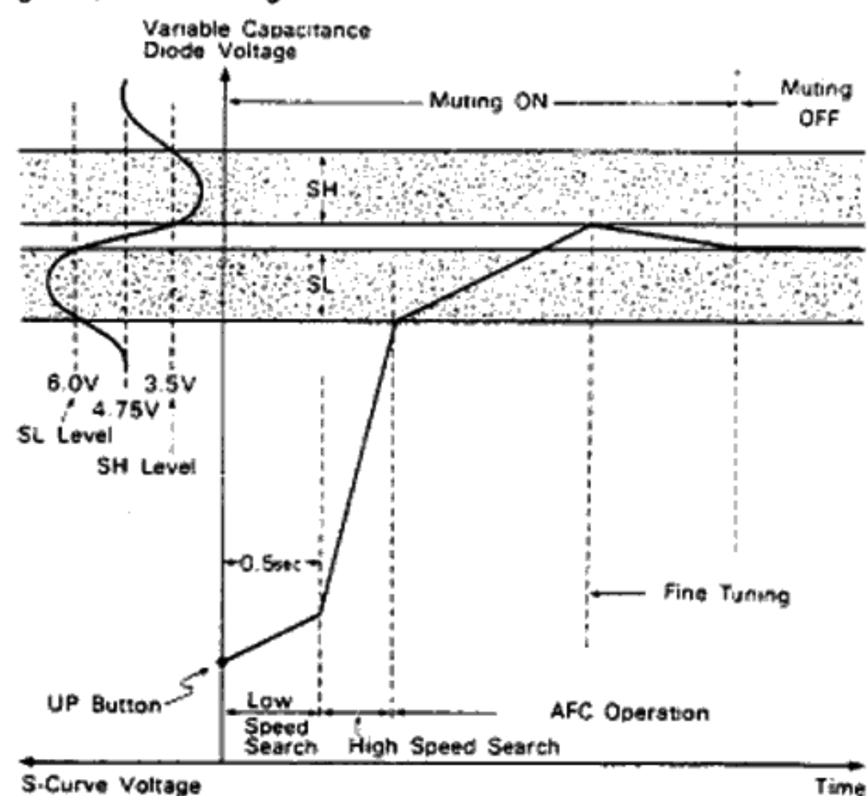
Fig.2-1 Search Tuning
