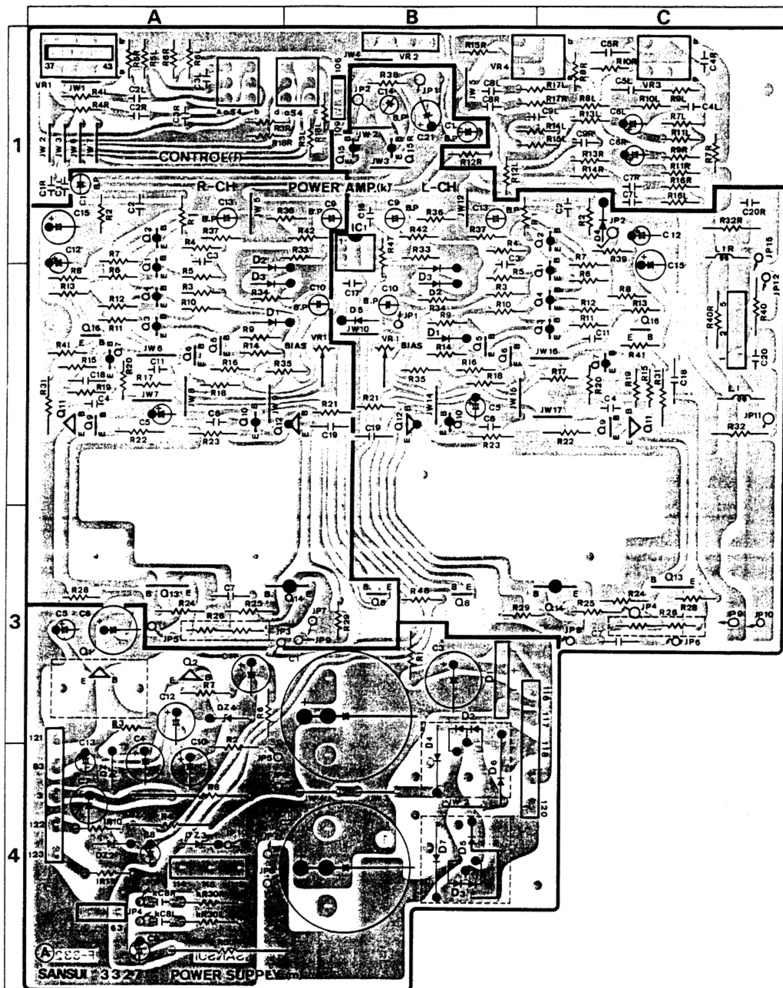
5-5. F-3327 Audio & Power Supply Circuit Board (Stock No. 07094901 = 5900Z/07096701 = 4900Z/00611101 = 3900Z) Component Side
