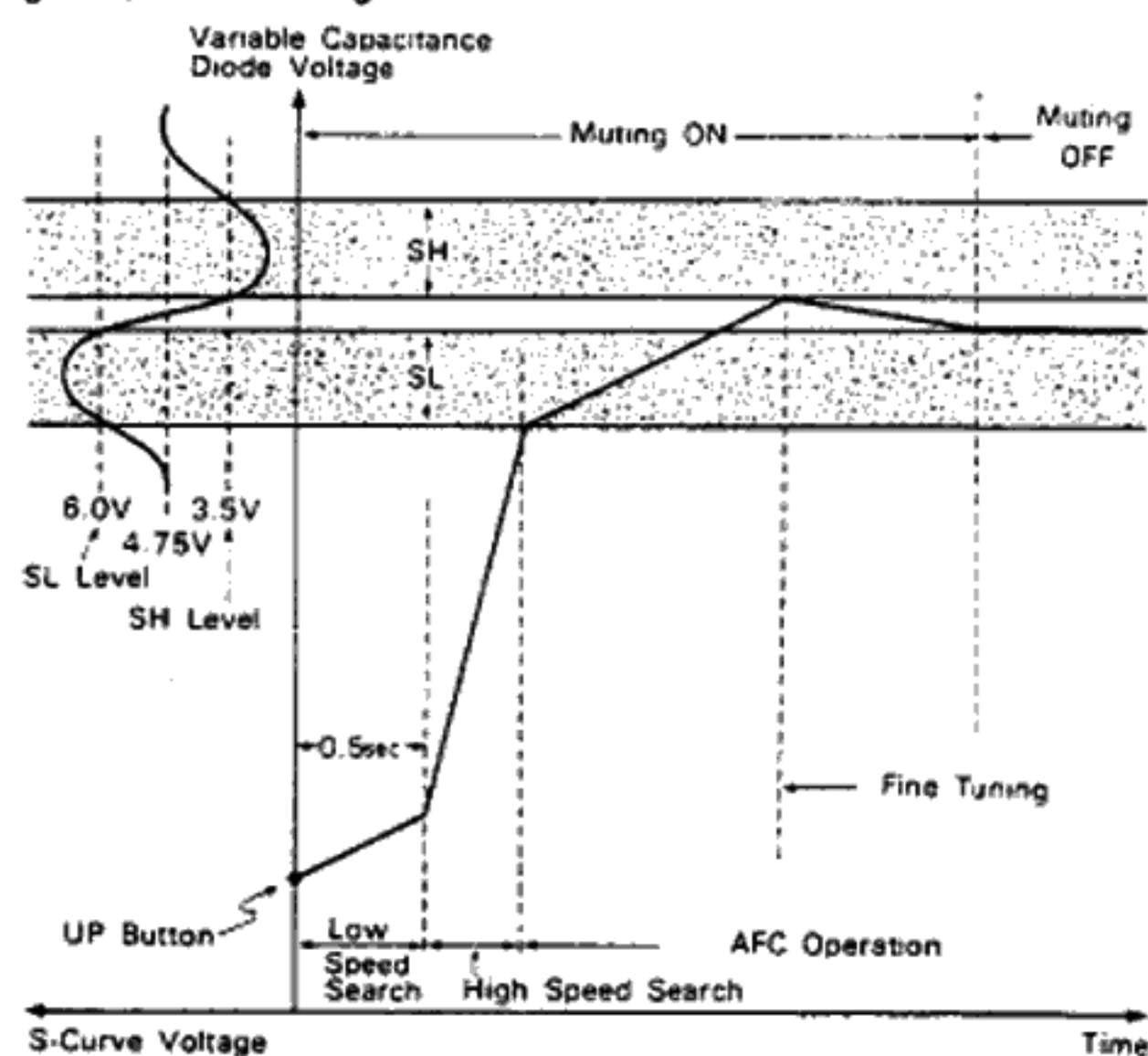
Fig.2-1 Search Tuning
