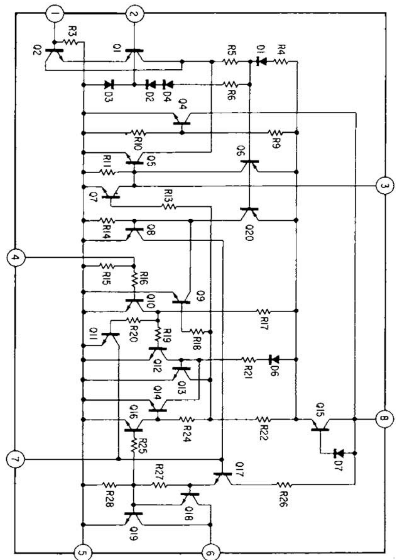
•µPC1237H (Speaker Protector IC)
