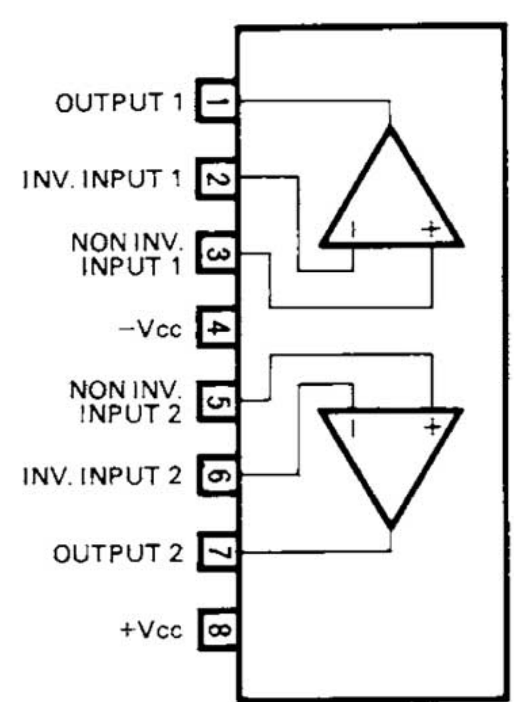
•M5220L (Audio PRE Amp. IC)
