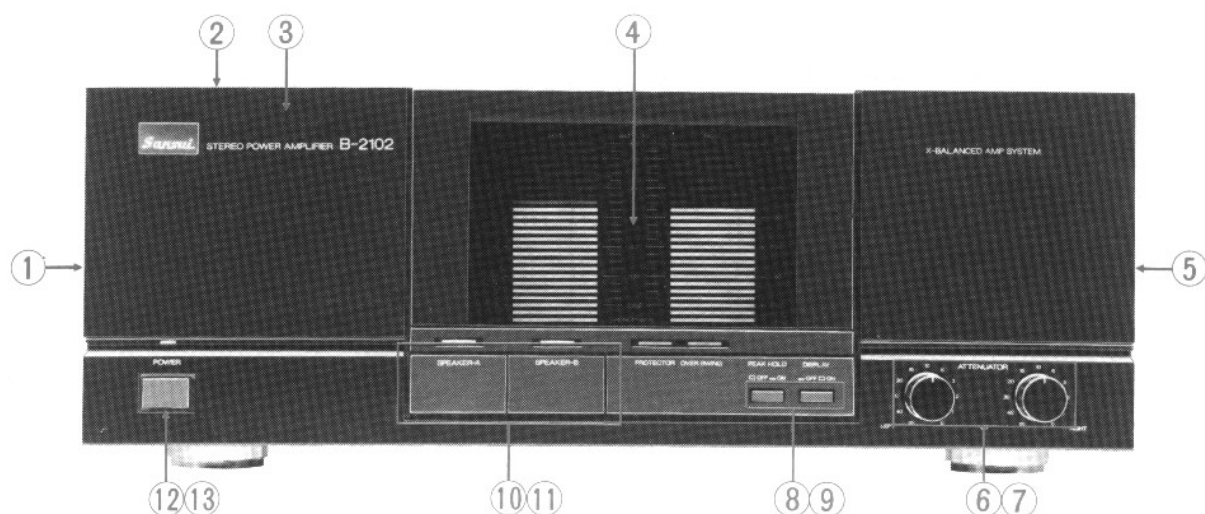
6-1. Front View
