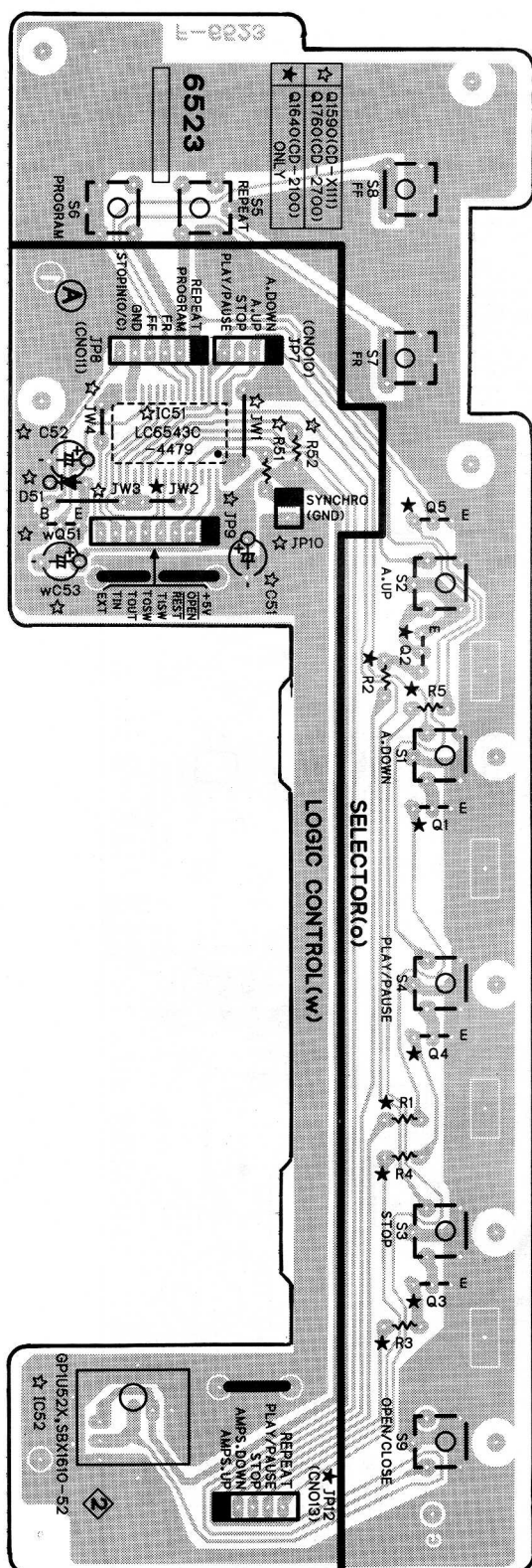
6-2. F-6523 Input Key Switch Board Component side
