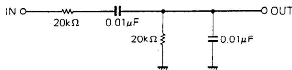
Band Pass Filter (BPF)
