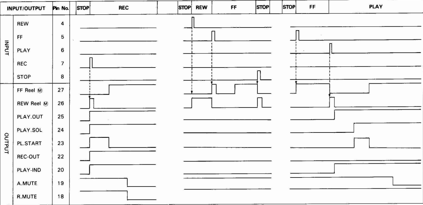
•Control IC (TC9310N-046, wIC1) Timing Chart (REC, REW→FF→STOP, FF→PLAY)
