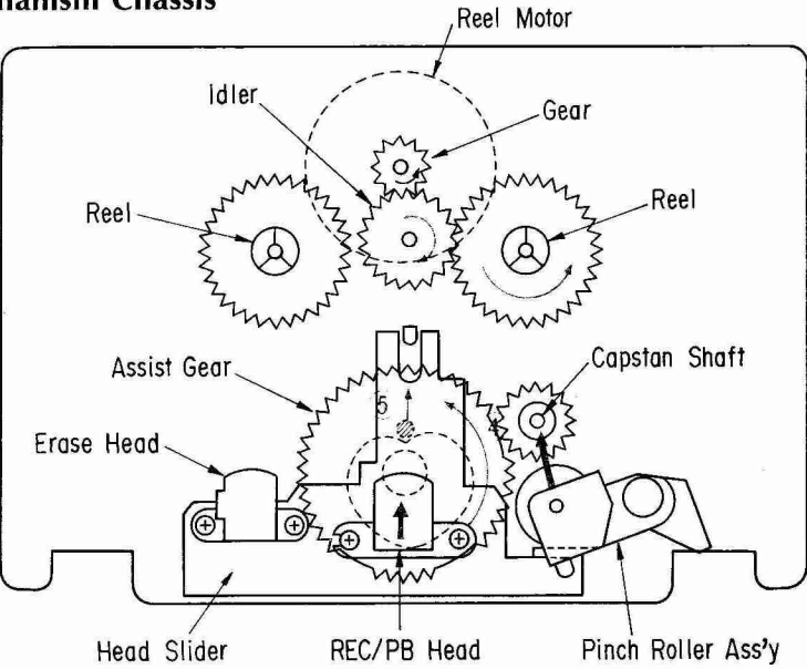
3-2. Front View of Mechanism Chassis
