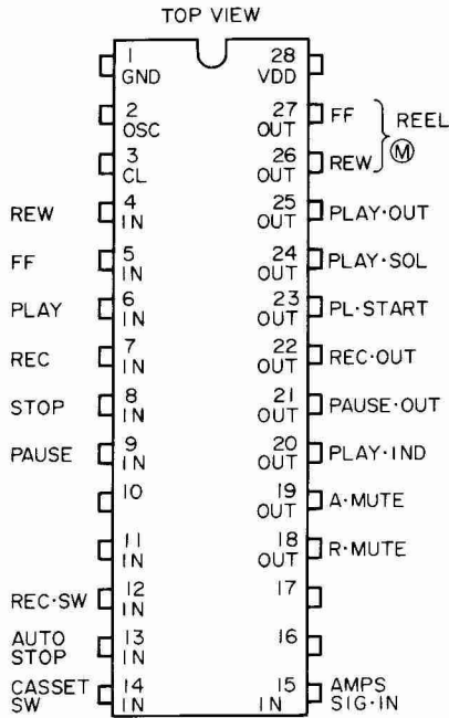
•Pin-connection
