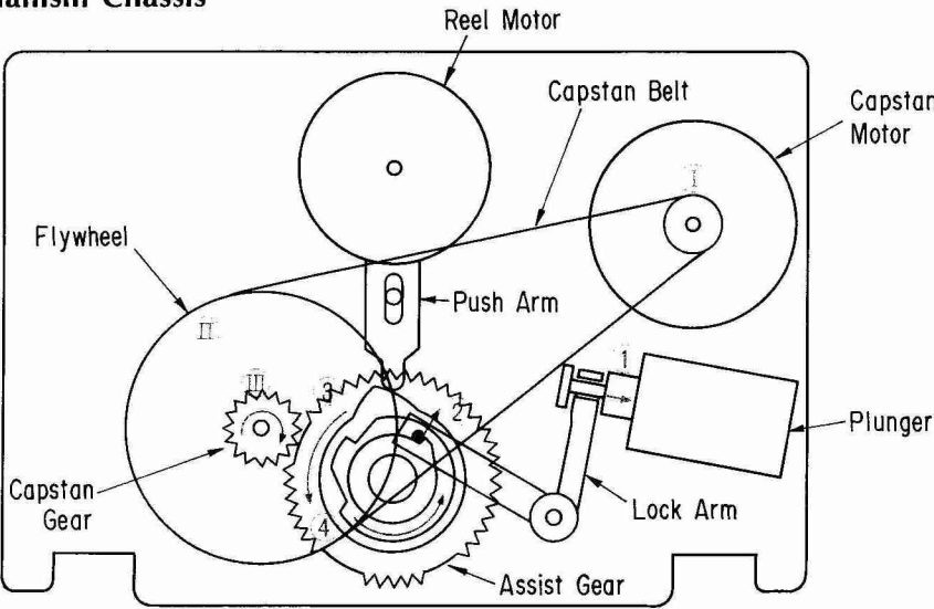
3-1. Rear View of Mechanism Chassis
