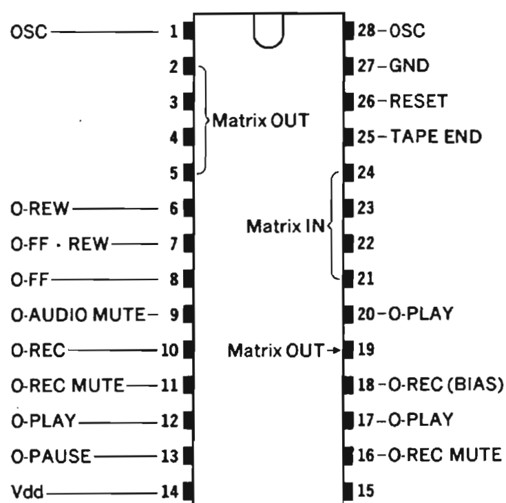
Fig. 2-3 Top View &amp; Pin function of IC D-554C
