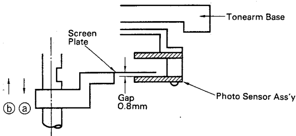
Fig. 3-1 Installation of Screen Plate (A) Side View of Screen Plate
