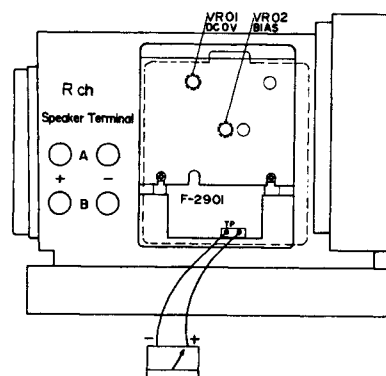
R-ch Side View of Power AMP Section
