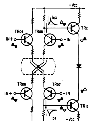
Fig. 2-5 (Fundamental of D.D. DC circuit)
