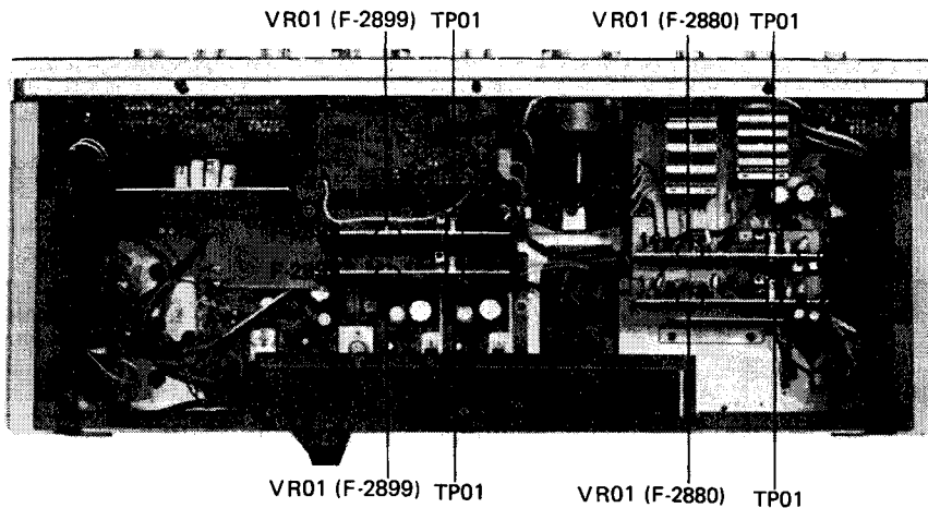
L-ch Side View of Power AMP Section
