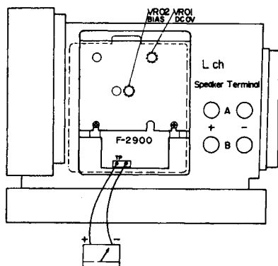
L-ch Side View of Power AMP Section
