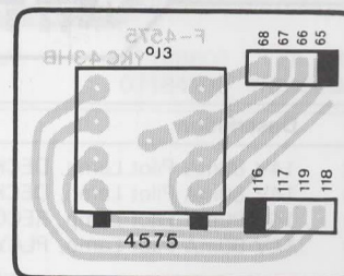
Component Side
