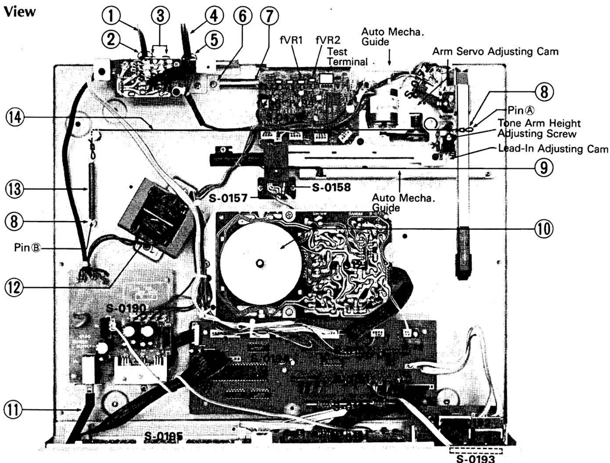
Parts List <Front View, Display Stage>
