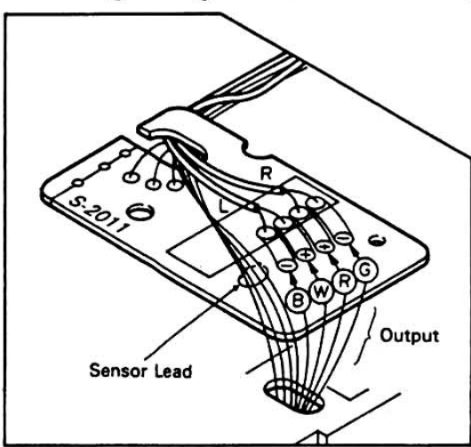
•Wiring Diagram of S-0211 (B Arm Side)
