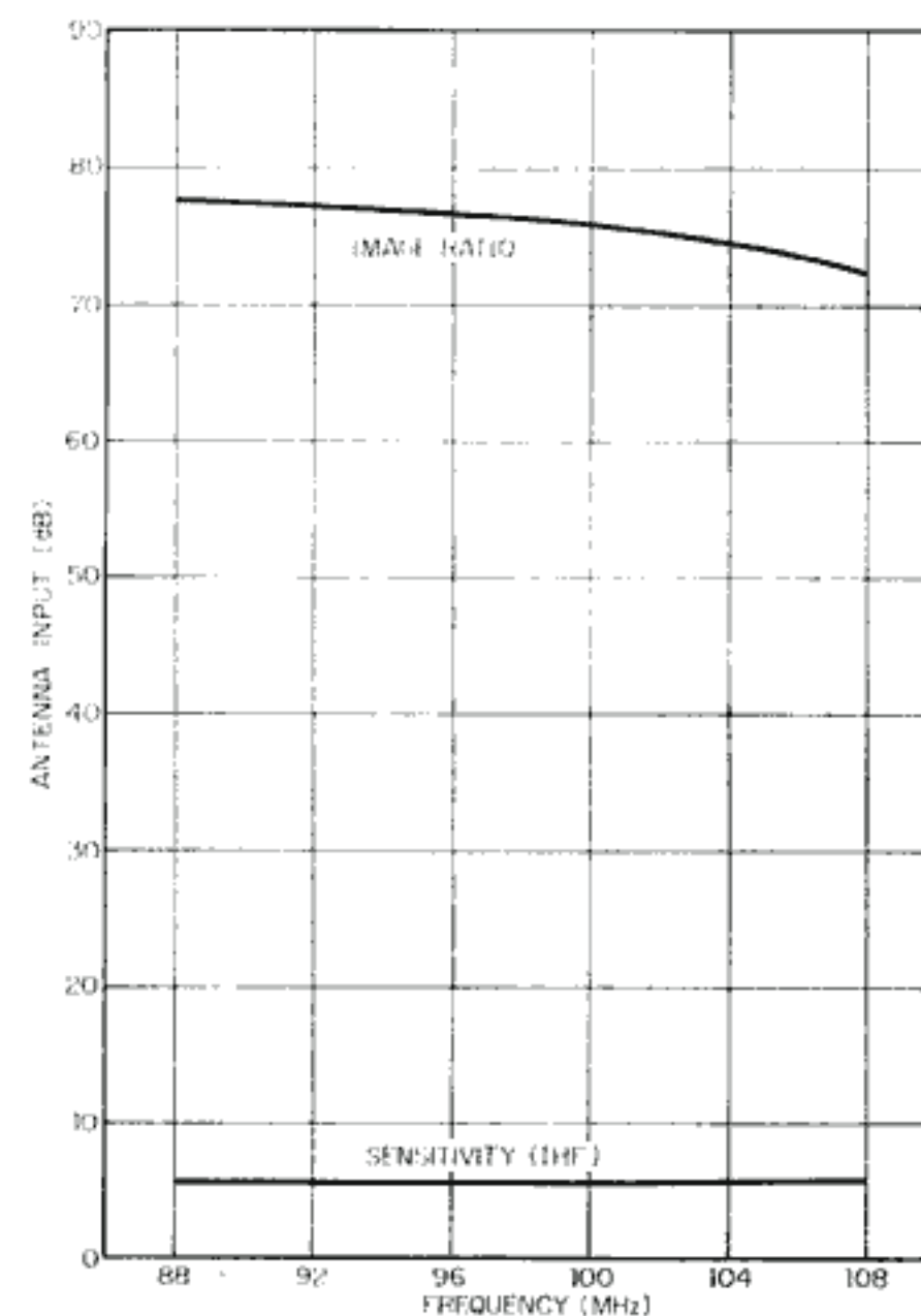
FM SENSITIVITY & IMAGE RATIO
