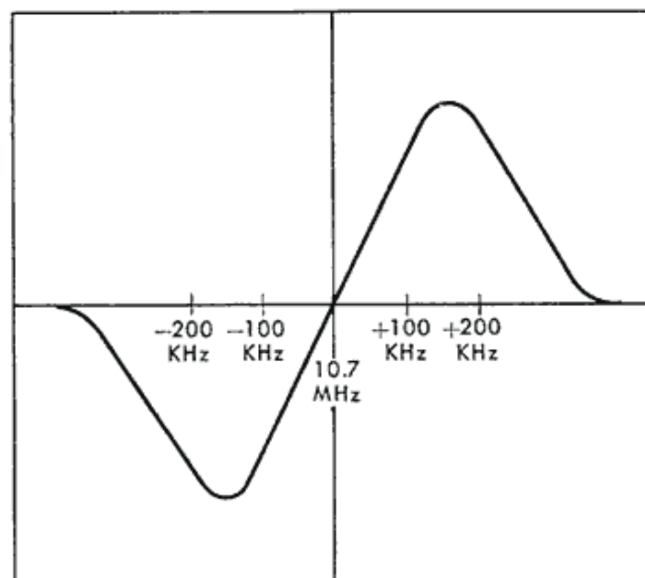
FM DISCRIMINATOR CHARACTERISTIC
