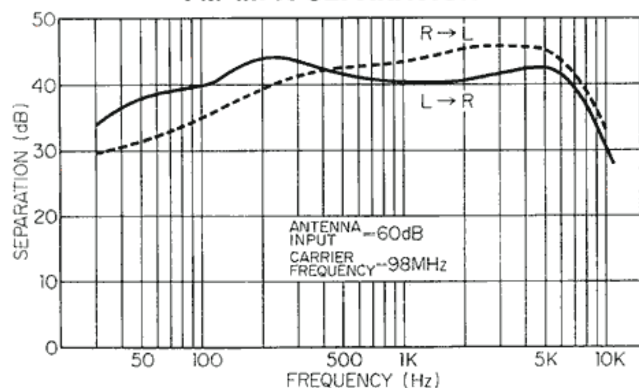
FM MPX SEPARATION
