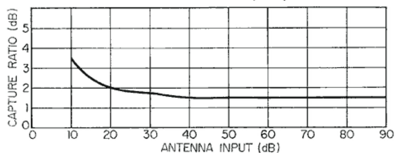
CAPTURE RATIO (IHF)
