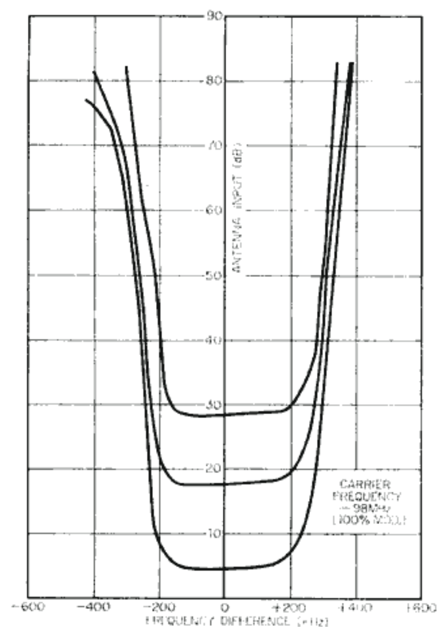
FM SELECTIVITY
