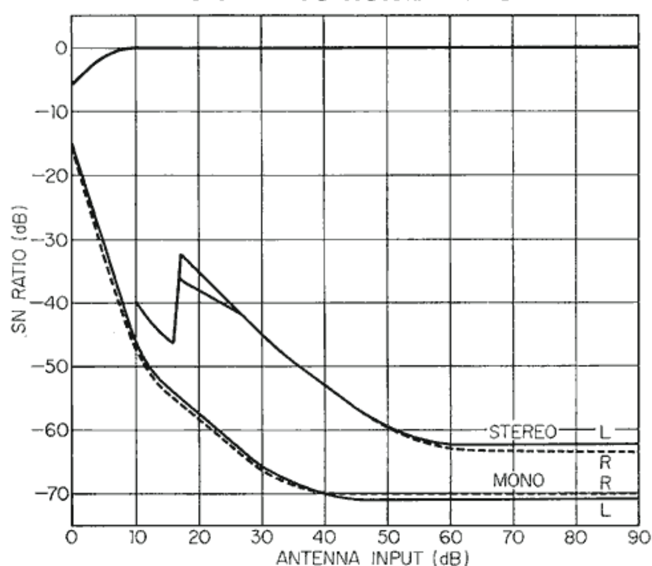
FM SIGNAL TO NOISE RATIO
