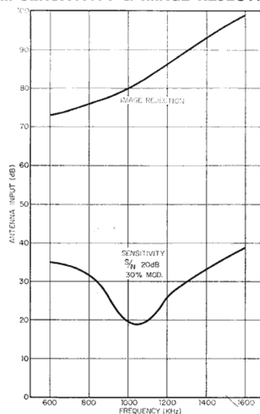
AM SENSITIVITY & IMAGE REJECTION
