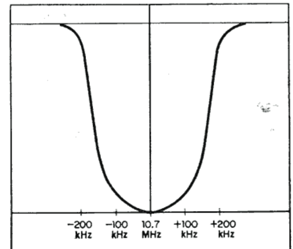
FM IF CHARACTERISTIC
