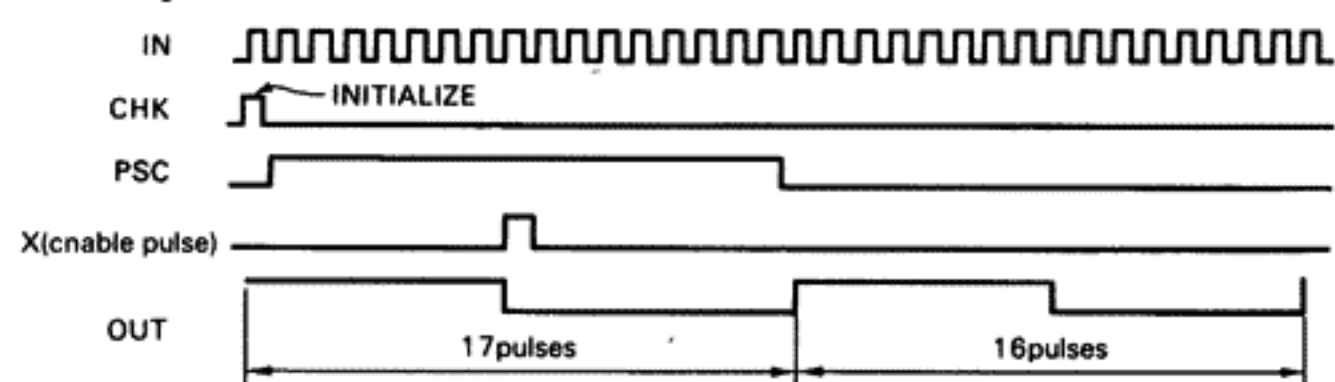
Timing Chart
