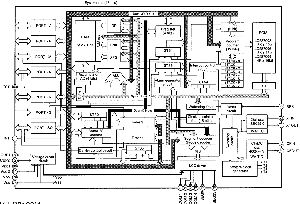
IC141 LB8108M
