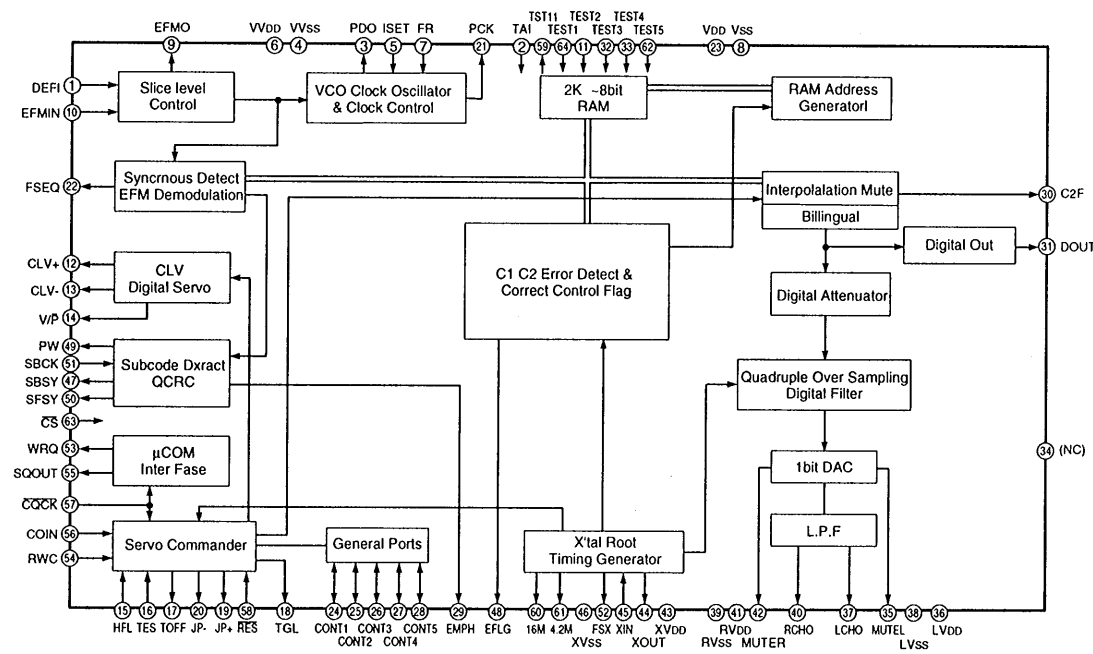
LC78622E (Digital Signal Processor)
