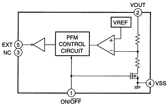
IC143 S-8322AIMP-DOI
