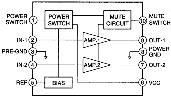
IC192 LA4533M
