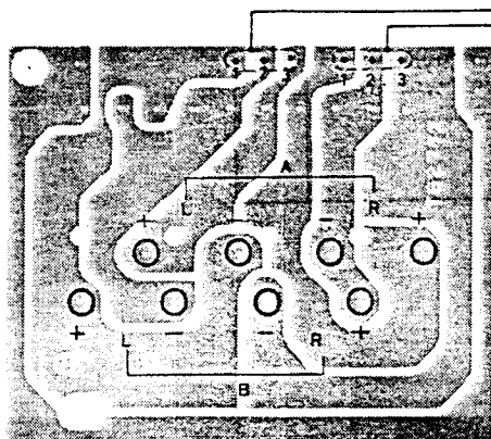
SPEAKER TERMINAL PCB
