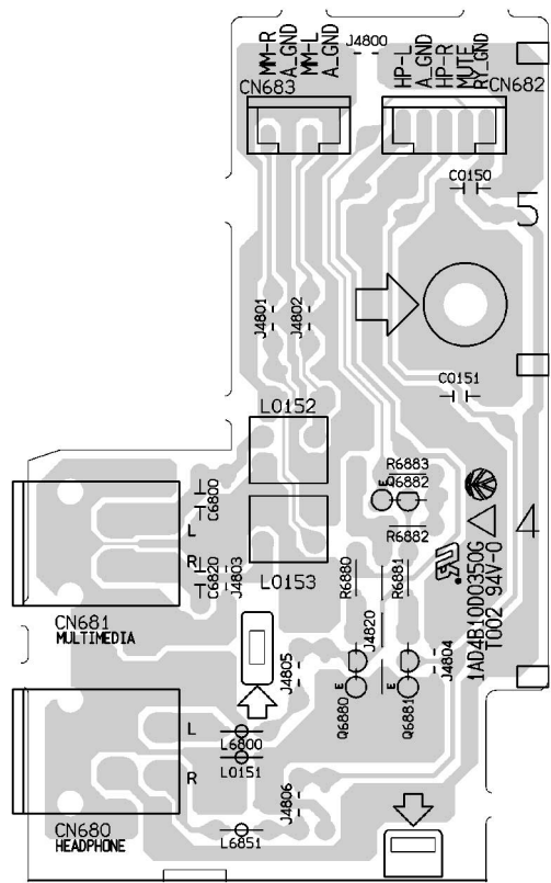
HEADPHONE P.W.BOARD
