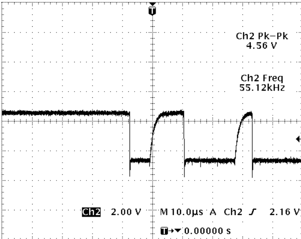
IC301 PIN 11
