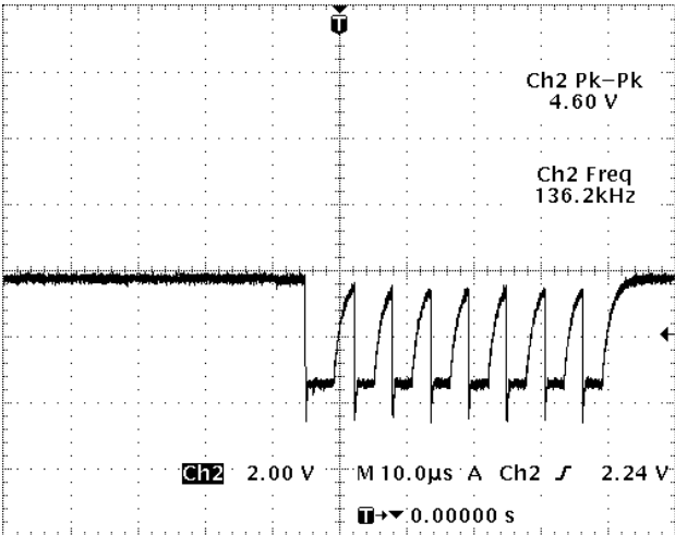
IC201 PIN 8
