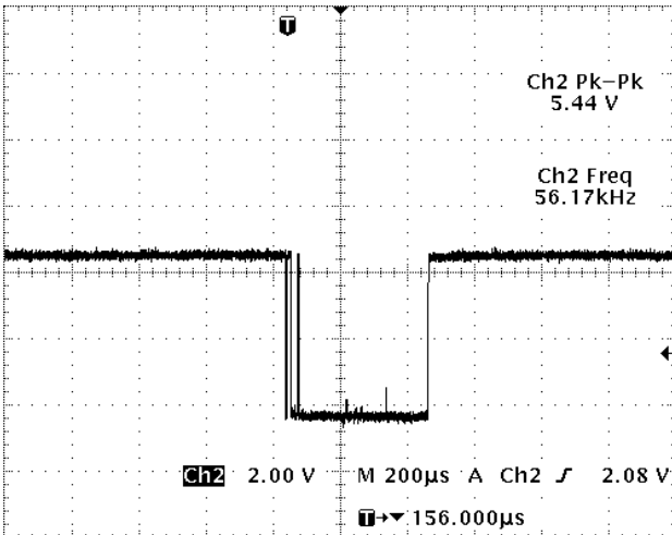
CP306 PIN 5
