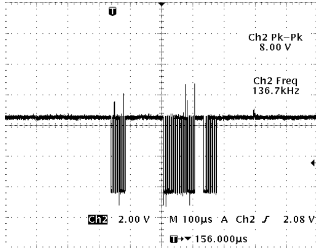
CP306 PIN 4
