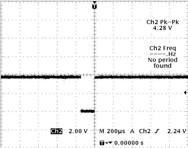
IC201 PIN 6
