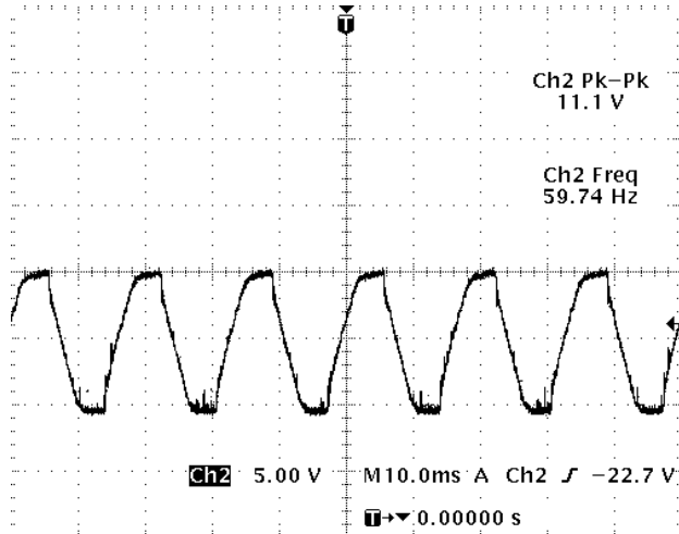
CP313 PIN 1
