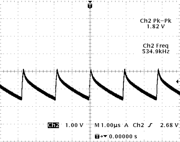
IC201 PIN 5
