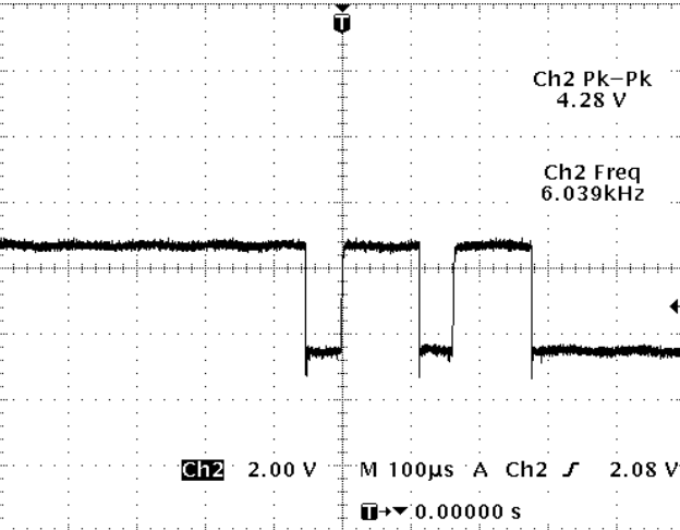
IC301 PIN 9
