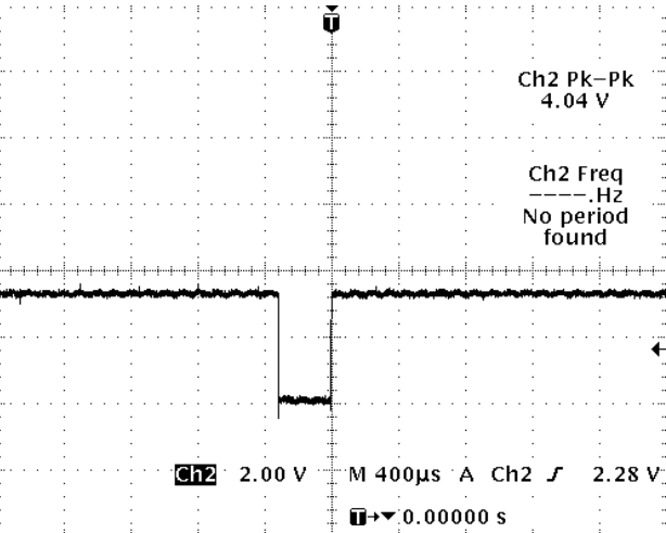
IC201 PIN 9
