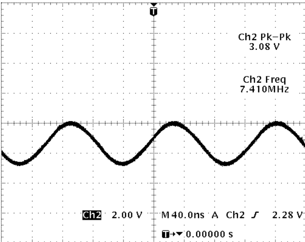
IC301 PIN 5
