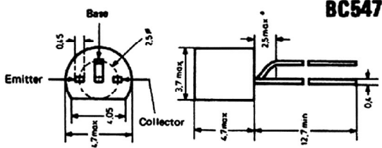
BC547
