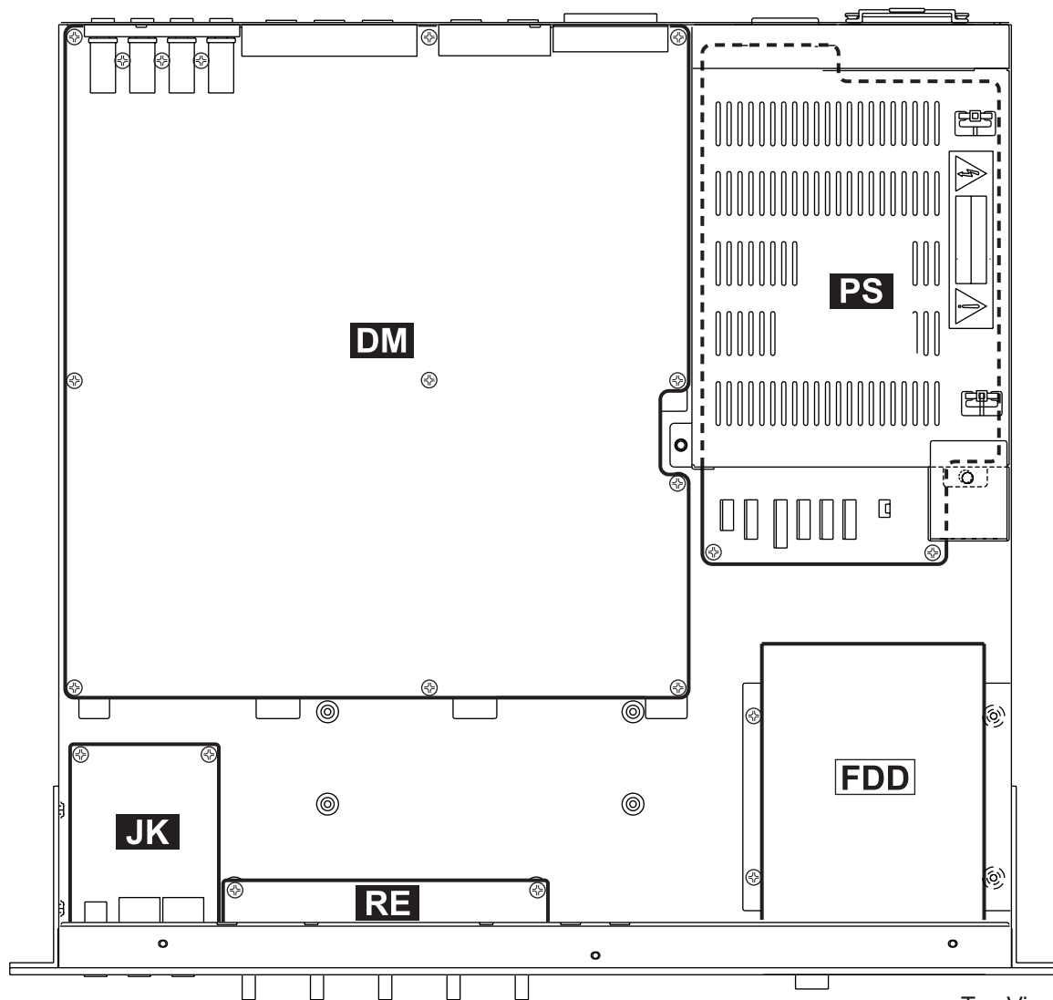
Top View (上面図)
