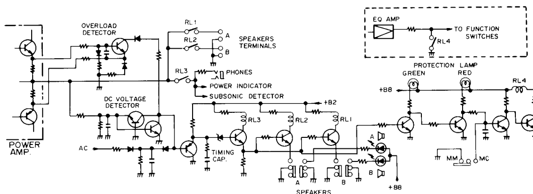
Fig. 4-6 Protection circuit
