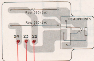
HEADPHONES JACK Ass'y
