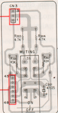
FM MUTING Ass'y
