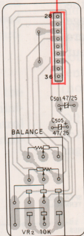
BALANCE CONTROL Ass'y
