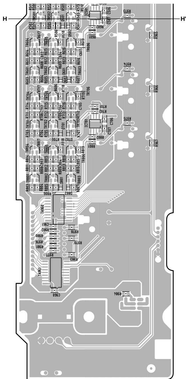
Pattern side
