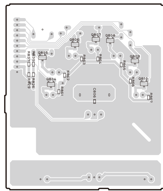
OPERATION (5) P.C.B. (Side B)
