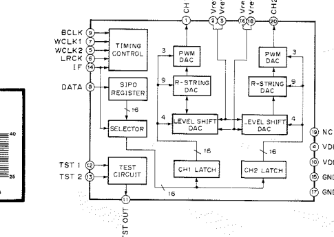
IC3 : LC9600AM 16 bit D/A Converter
