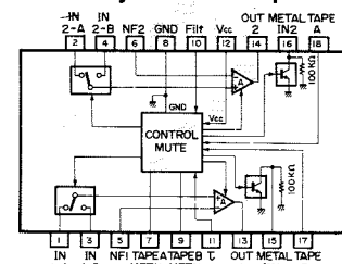
IC401 : BA316BL Dual Playback Preamplifier
