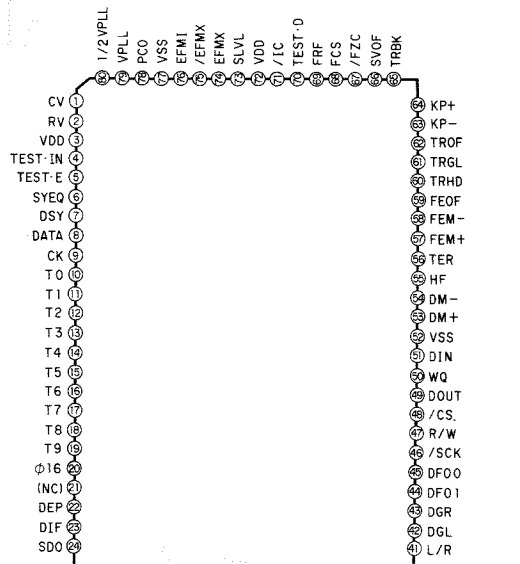
IC2 : YM7121C Signal Processor & Controller
