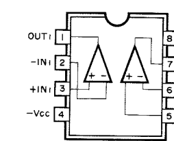
IC4, 5 : NJM4560M Dual OP-Amp
