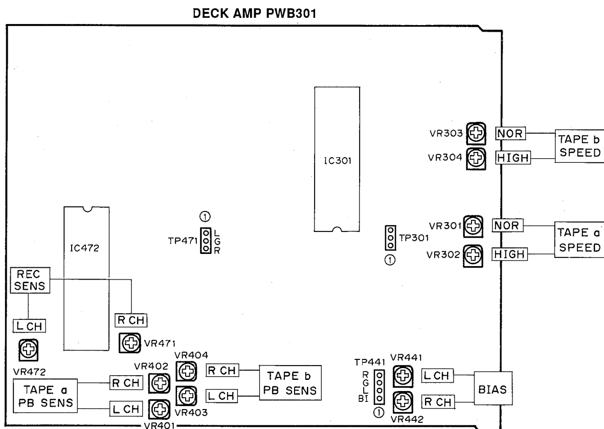
Figure 6-4 ADJUSTMENT POINTS
