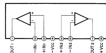
IC701 ~ 704, 707, 801, 803 : M5218AL Dual OP-Amp
