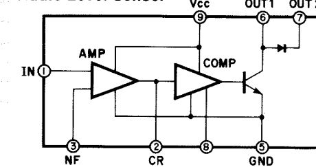
IC402 : LA2000 Audio Level Sensor
