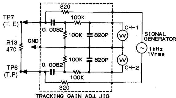
Figure 5-4 TRACKING GAIN
