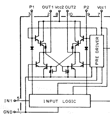
IC851, 852 : LB1641 Motor Driver
