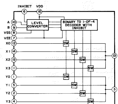
IC706, 802 : MC14052BC Differential 4-Channel Multiplexer/Demultiplexer
