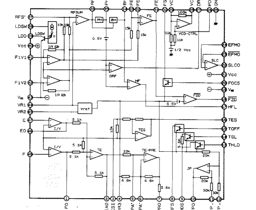
IC9 : LA9200M Servo Amp
