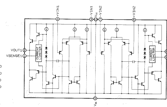
IC11, 12 : LA6515 Dual Power Operational Amp
