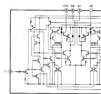
IC11, 12 : LA6515 Dual Power Operational Amp
