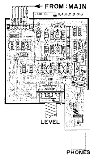
Operation Circuit Board (2)
