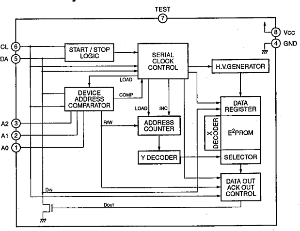
IC320 : S-24C01ADP Electrically Erasable PROM
