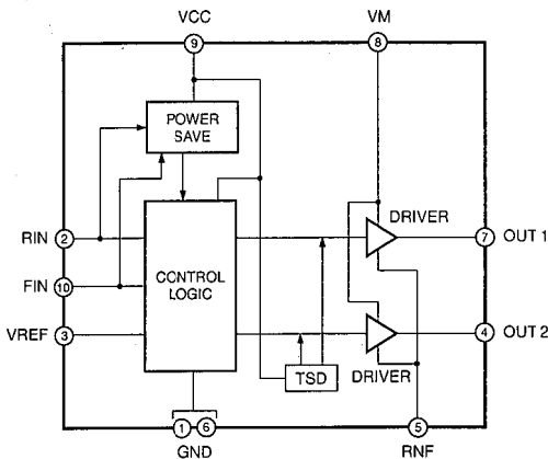
IC400 : BA6286 Motor Driver
