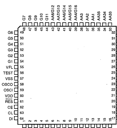
IC303 : LC75711NE FL Driver
