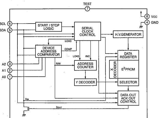
IC302 : S-24C01ADP Electrically Erasable PROM
