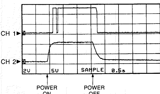
Point ② CH 1 : Pin 24 of IC311 CH 2 : Collector of Q204 V : 2V/div (CH 1) V : 5V/div (CH 2) H : 0.5sec/div DC range 1 : 1 probe
