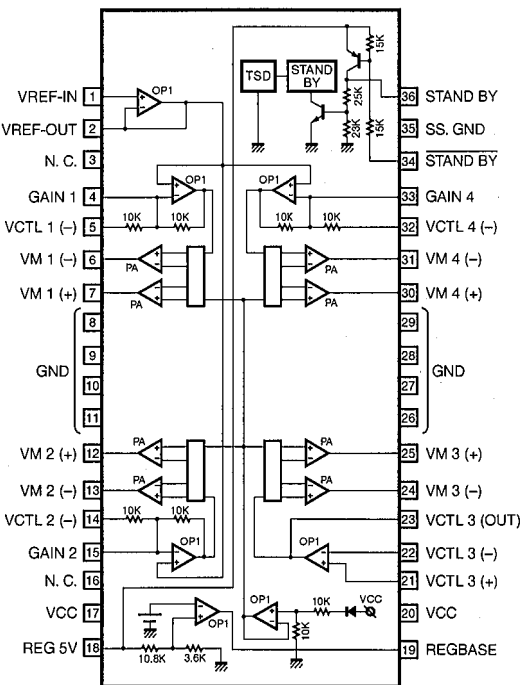
IC2 : M56748FP 4-Channel BTL Driver
