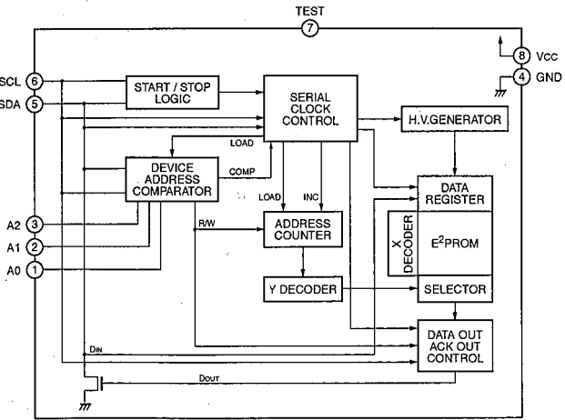
IC302 : S-24C01ADP Electrically Erasable PROM
