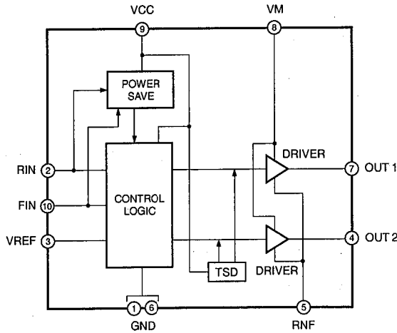
IC303 : BA6286 Motor Driver
