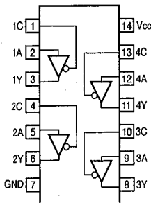
IC10 : HD74HC125P Quad 3 State Bus Buffers
