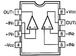
IC104, 105 : NJM5532D IC102, 103 : NJM2068D-D IC120 : BA15218 Dual Op-Amp
