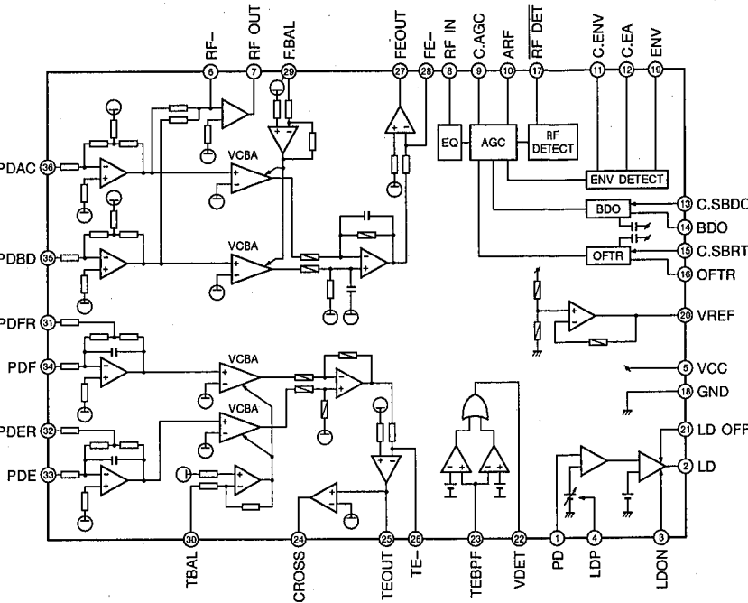
IC2 : LA6536M 4-Channel BTL Driver
