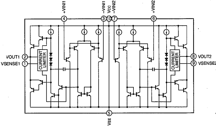
IC304 : LA6510 Dual Power Operational Amp
