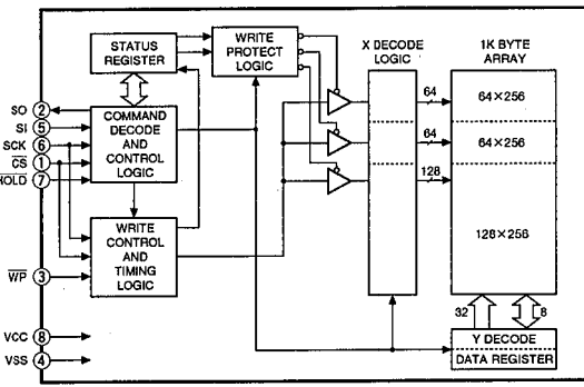
IC320 : X25642D Electrically Erasable PROM
